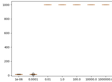
(b) Number of misclassified adversarial configurations (100 displacements)
