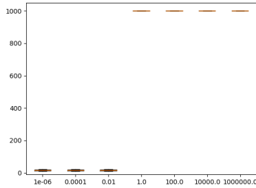
(a) Number of misclassified adversarial configurations (20 displacements)
