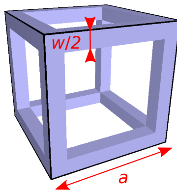
Figure 2. Unit cell of a simple cubic lattice composed of wire cubes assembled side by side (Dul’nev model). In the 3D-lattice, the width of the cube edges is w .
