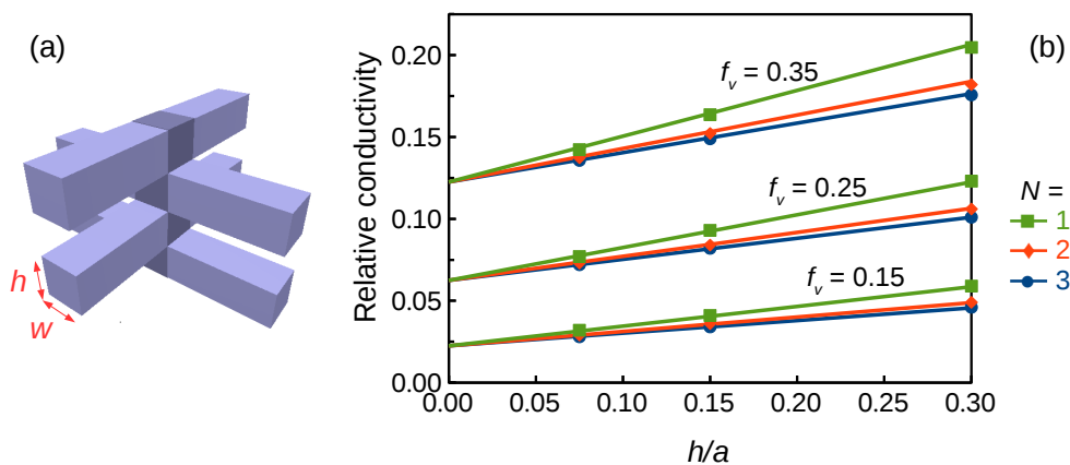
Figure A1. (a) Unit cell of the woodpile structure composed of N = 2 layers ( w/a = 0.15 , h/a = 0.15 ). The part in deep color represents the core column. (b) Plot of \kappa_e/\kappa_m versus the height to length ratio h/a of the bars for three volume-filling fractions f_v = w/a and for N = 1, 2 , and 3 layers. The symbols are from Table 1 and the full lines are from Equation (A5).
