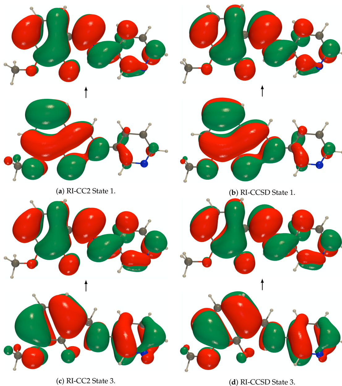
Figure A2. def2-TZVPD NTOs (holes below the arrows and particles above them, the red (green) lobes are the positive (negative) ones) of the isolated PYV3 [PYV3] keto form (isovalue of 0.02 a.u.).
