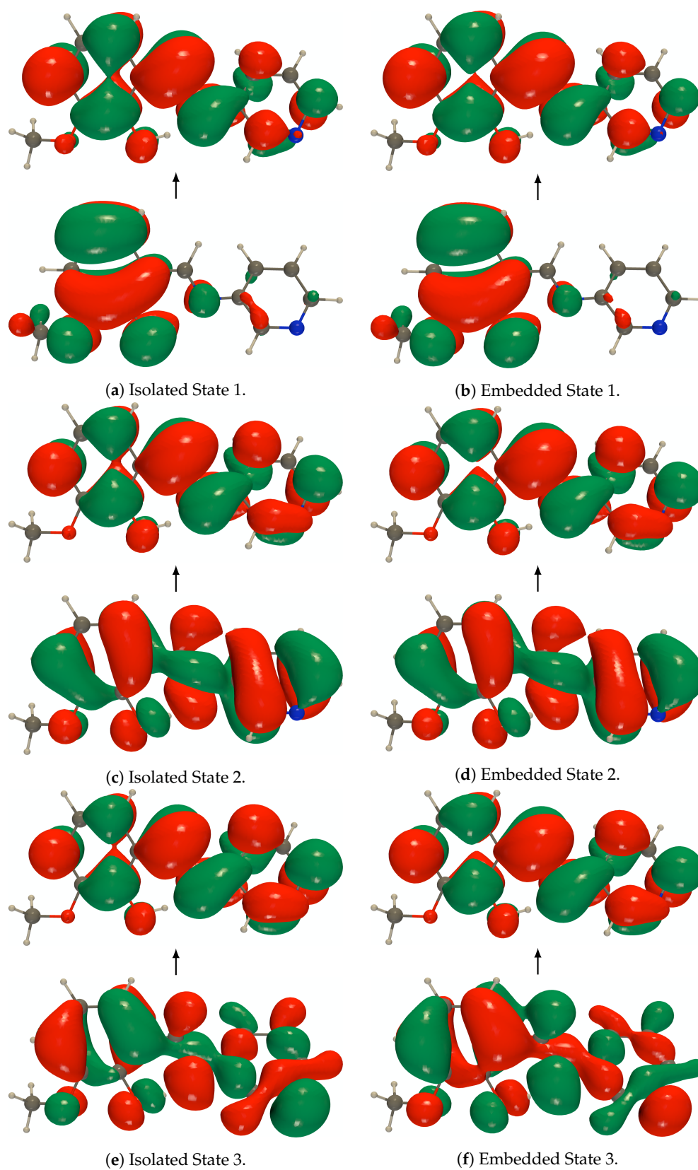
Figure A5. RI-CC2/def2-TZVPD NTOs (holes below the arrows and particles above them, the red (green) lobes are the positive (negative) ones) of the isolated and embedded PYV3 [PYV3] enol form (isovalue of 0.02 a.u.).
