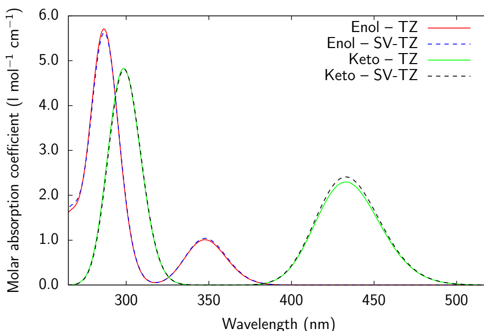
Figure 9. RI-CC2 composite (SV-TZ, dashed lines) and def2-TZVPD (TZ, full lines) spectra for the embedded heteromers of PYV3 · SA and PYV3 · FA1.
