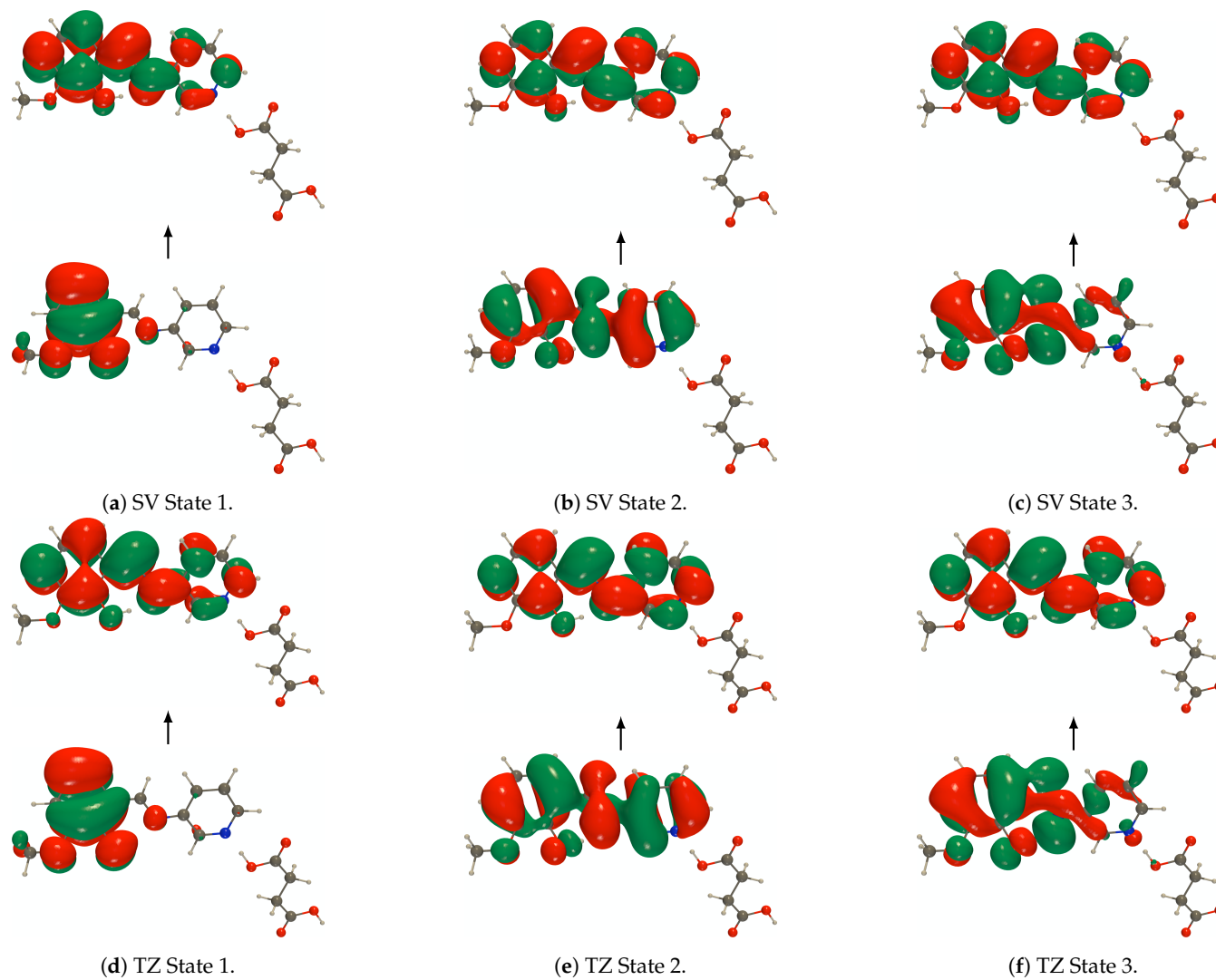
Figure A7. RI-CC2 def2-SVPD (SV) and def2-TZVPD (TZ) NTOs (holes below the arrows and particles above them, the red (green) lobes are the positive (negative) ones) of the embedded PYV3 + SA [PYV3 · SA] enol form (isovalue of 0.02 a.u.).
