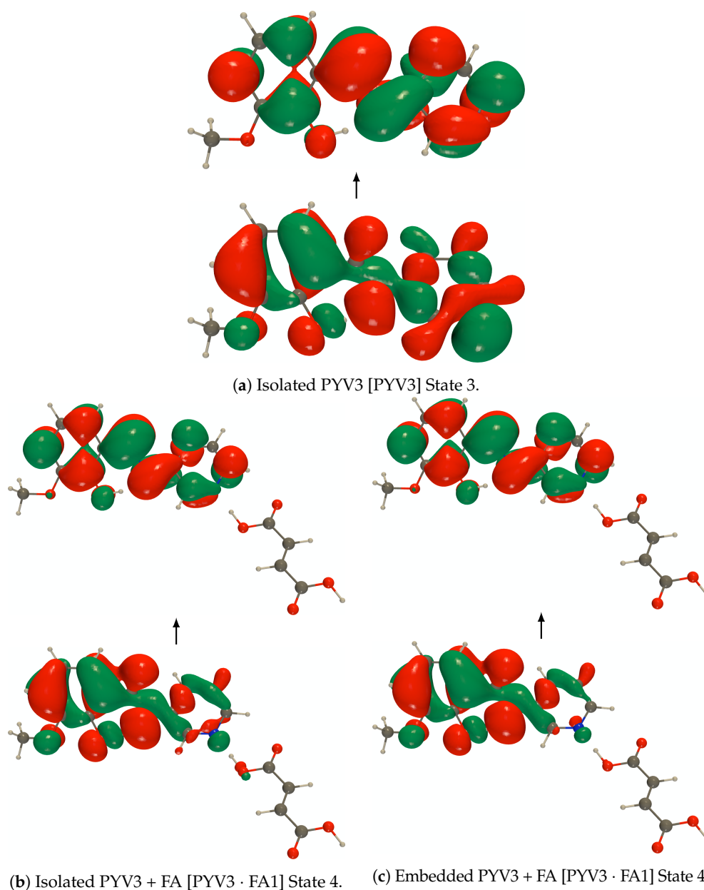
Figure A4. RI-CC2/def2-TZVPD NTOs (holes below the arrows and particles above them, the red (green) lobes are the positive (negative) ones) of the 3rd excited state of the isolated PYV3 [PYV3] enol form and of the 4th excited state of the isolated and embedded PYV3 + FA [PYV3 · FA1] (isovalue of 0.02 a.u.).
