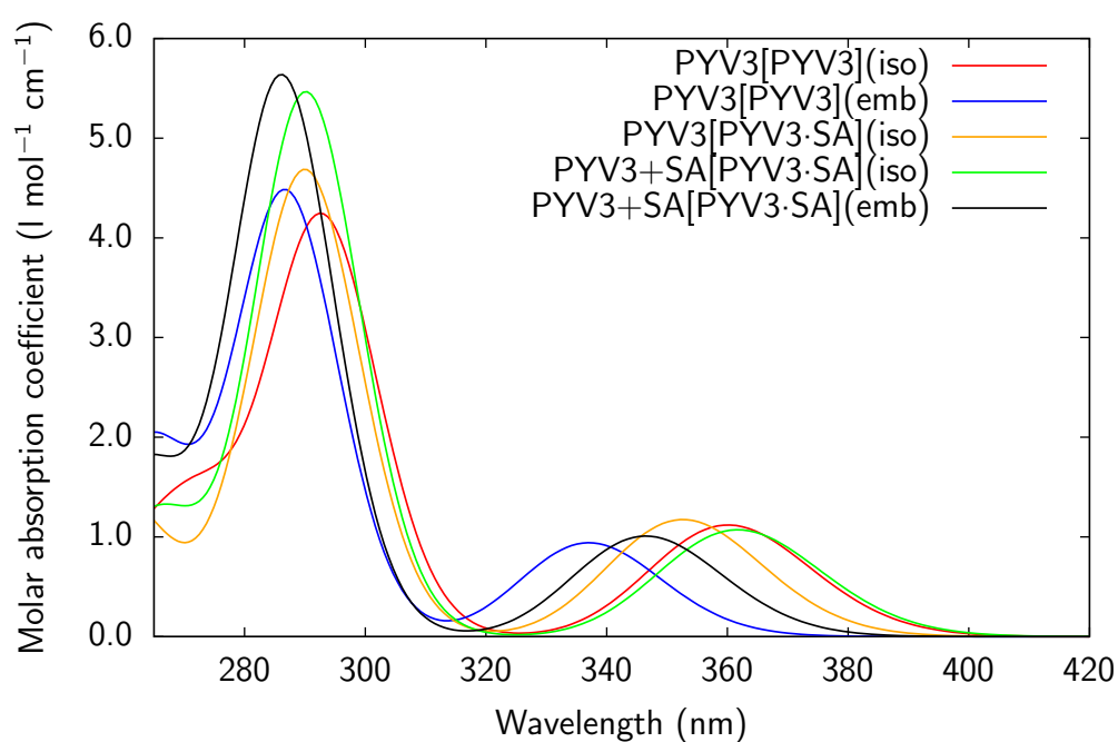
(a) Enol.
