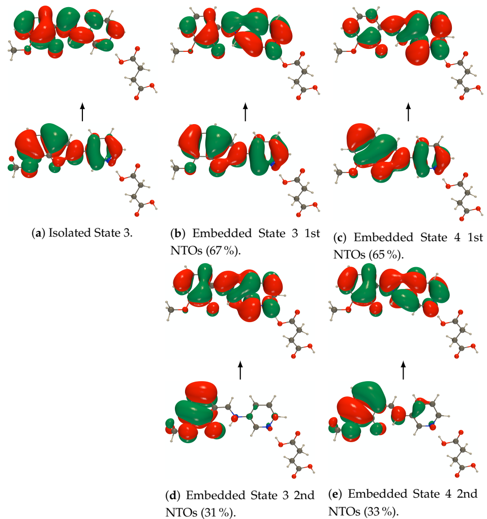
Figure 8. RI-CC2/def2-TZVPD NTOs (holes below the arrows and particles above them, the red (green) lobes are the positive (negative) ones) of the 3rd isolated keto form of PYV3 + SA [PYV3 · SA] and of the 3rd and 4th excited states of the embedded one (isovalue of 0.02 a.u.).
