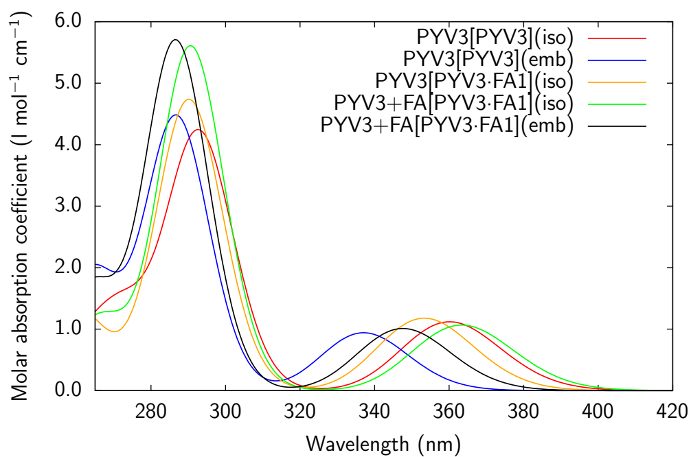
(a) Enol.
