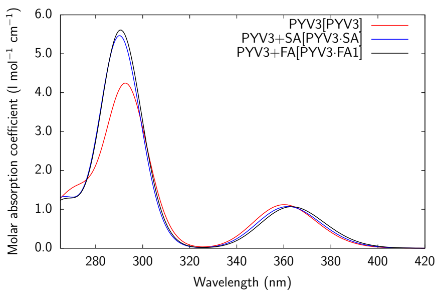
(a) Enol.
