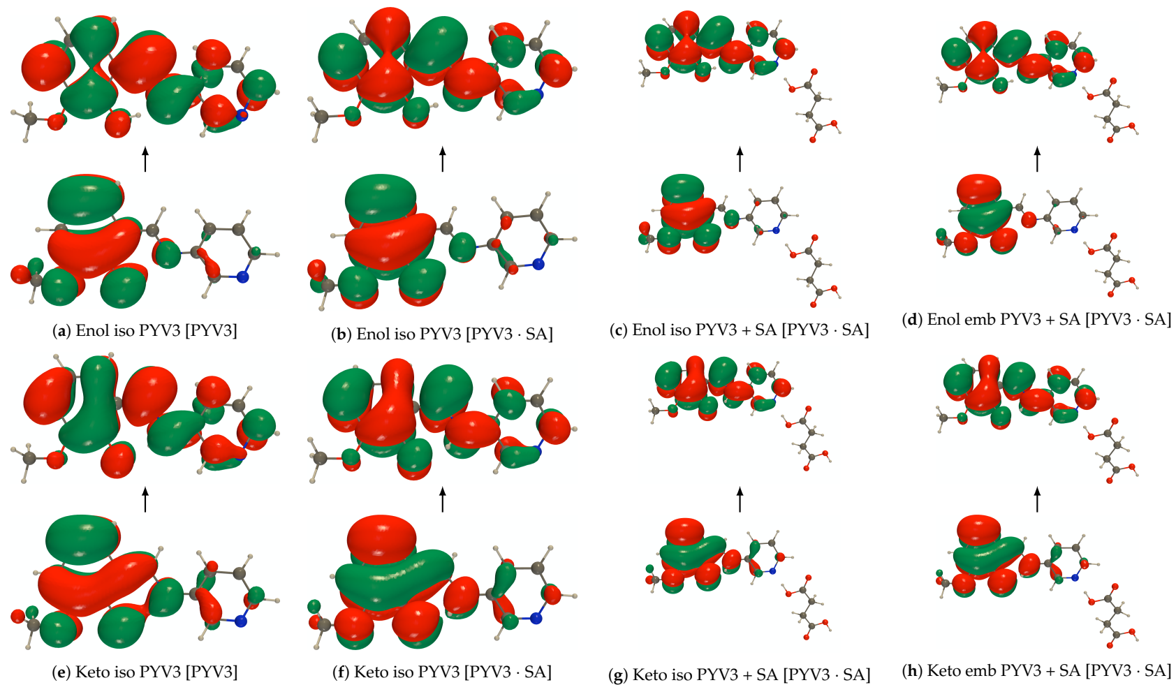
Figure 7. RI-CC2/def2-TZVPD NTOs (holes below the arrows and particles above them, the red (green) lobes are the positive (negative) ones) of the first excited state of isolated PYV3 [PYV3] and the various models of PYV3 · SA (isovalue of 0.02 a.u.). “Iso” stands for isolated while “emb” for embedded in crystal field point-charges.
