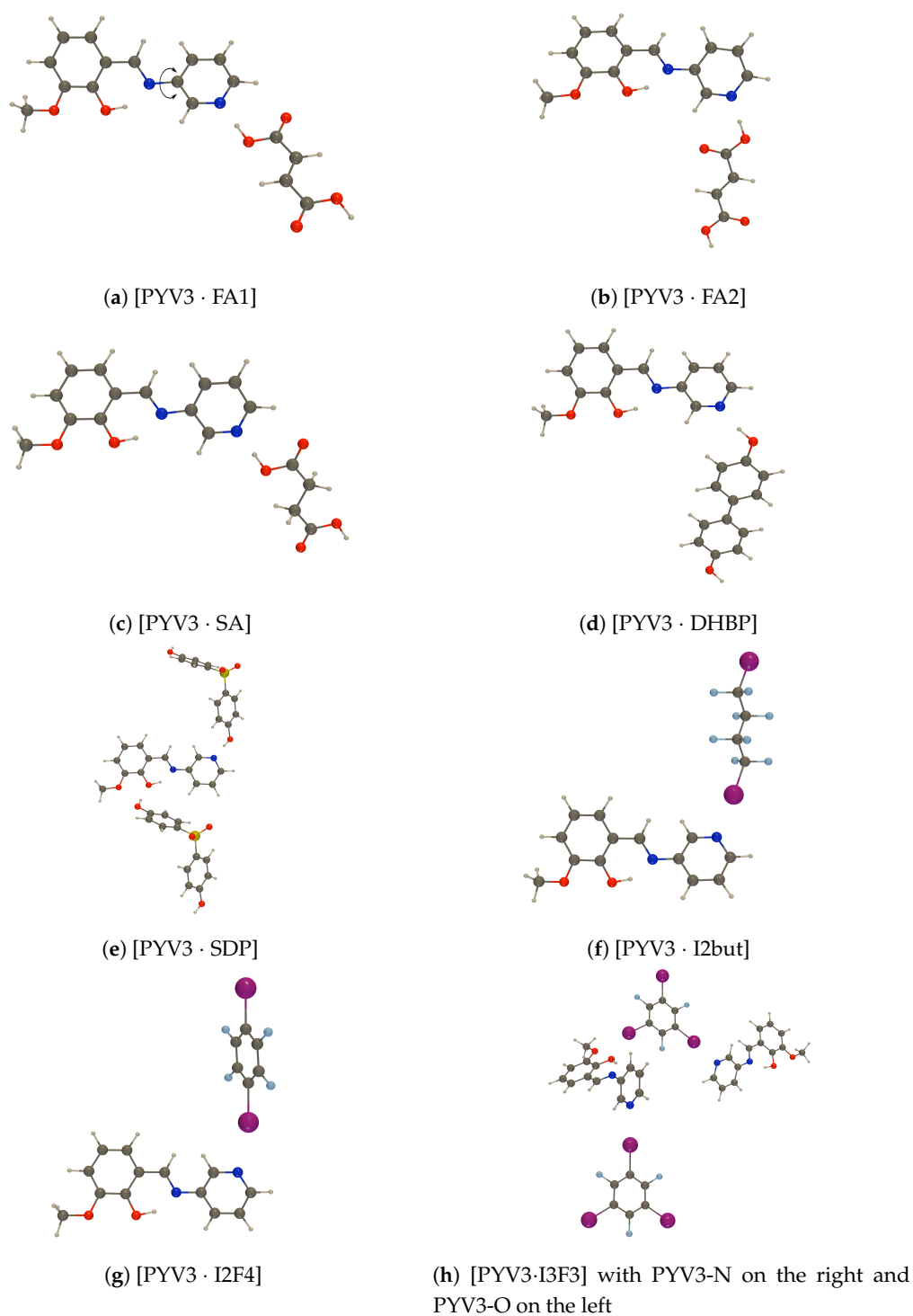
Figure 1. Representation of the PYV3-coformer synthons as extracted from the co-crystal structure optimized at the PBC/PBESol0/6-31G(d,p)/I(LANL2DZ) level of approximation. Here, the enol form was considered for all co-crystals. The corresponding references to the X-ray diffraction structures are also provided. In the case of a , an arrow has been added to define the pyridine torsion angle.
