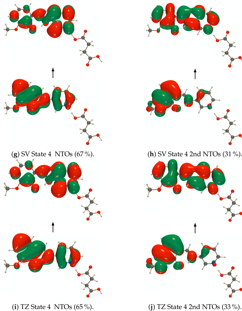
Figure A8. RI-CC2 def2-SVPD (SV) and def2-TZVPD (TZ) NTOs (holes below the arrows and particles above them, the red (green) lobes are the positive (negative) ones) of the embedded PYV3 + SA [PYV3 · SA] keto form (isovalue of 0.02 a.u.).
