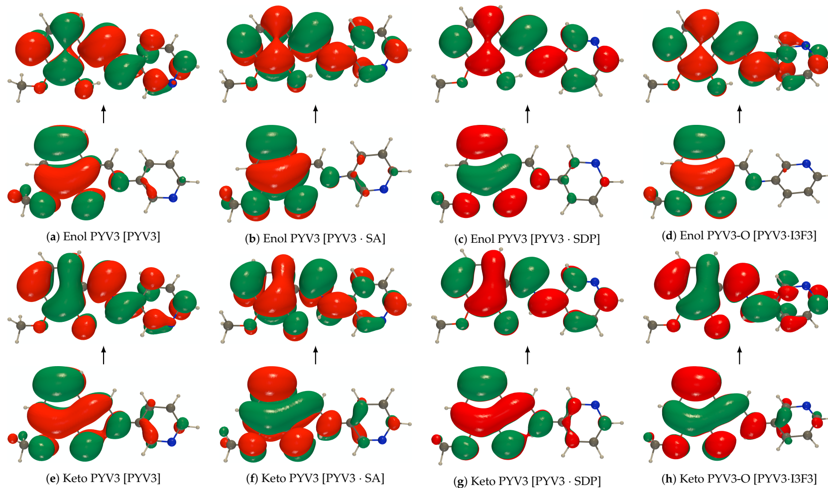
Figure 6. RI-CC2/def2-TZVPD NTOs (holes below the arrows and particles above them, the red (green) lobes are the positive (negative) ones) of the first excited state of isolated monomers of PYV3, PYV3 · SA, PYV3 · SDP, and PYV3-I3F3 (isovalue of 0.02 a.u.).
