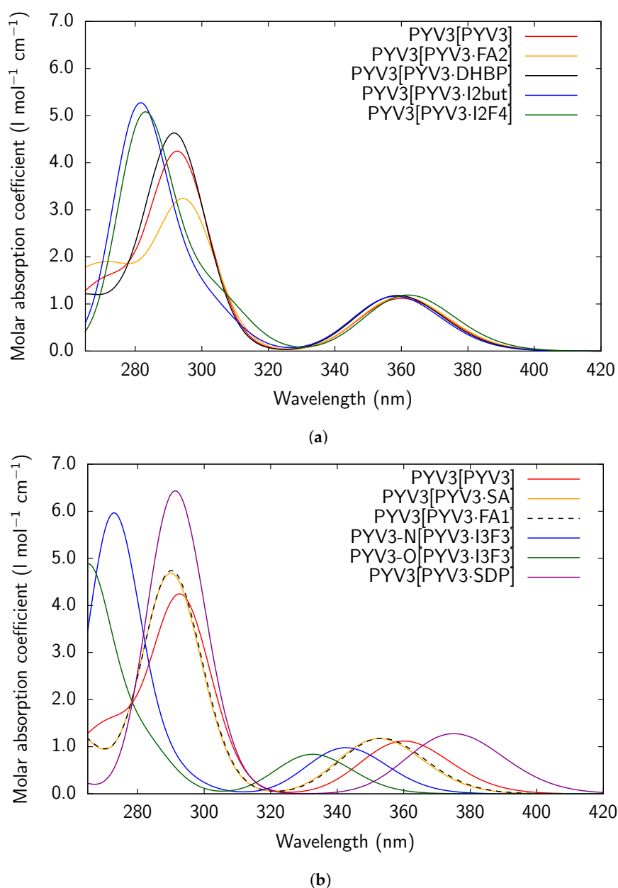
Figure 2. RI-CC2/def2-TZVPD UV/Vis absorption spectra of isolated monomers of all-enol crystals (PYV3 [PYV3 · XXX]). For clarity, the spectra have been splitted in two parts, see (a) and (b).
