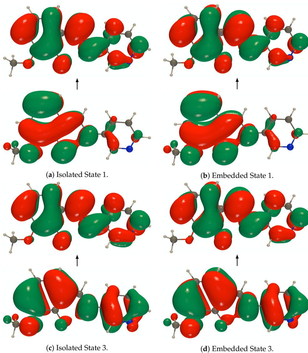
Figure A6. RI-CC2/def2-TZVPD NTOs (holes below the arrows and particles above them, the red (green) lobes are the positive (negative) ones) of the isolated and embedded PYV3 [PYV3] keto form (isovalue of 0.02 a.u.).
