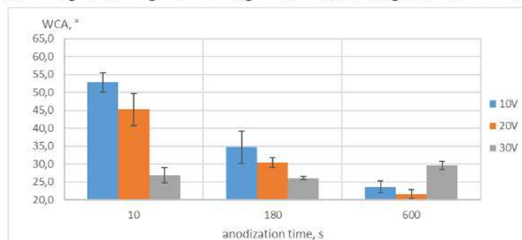
Fig. 2 : water contact angle (WCA) obtained for 9 anodisation conditions.
