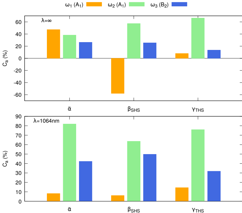
FIG. 2: Missing mode analysis [ C_a , %] ( \omega_1 , A_1 bending; \omega_2 , A_1 symmetric stretching; \omega_3 , B_2 antisymmetric stretching) to the static (top) and dynamic ( \lambda = 1064 \text{ nm} , bottom) total vibrational contributions to \bar{\alpha} , \beta_{SHS} , and \gamma_{THS} ), as computed at the CCSD/d-aug-cc-pVTZ level.
