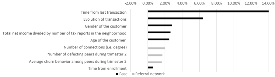
Figure 5: AUC Variable importance of metrics for base+referral model - random forest classifier
