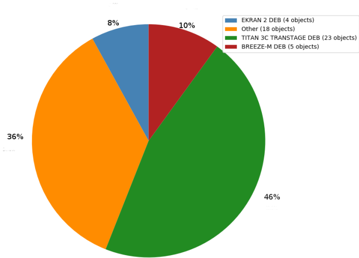
Figure 2.1 – Percentage of space debris in the geostationary region corresponding to different breakups that took place up to the date 2017/10/22. The objects gathered in the category "Other" are individuals objects not related to one of the major breakups summarized in Table 2.1.
