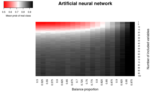
Figure 5.11 – Mean probabilities of real class depending on the number of inserted variables and the balance proportion between classes for artificial neural network.
