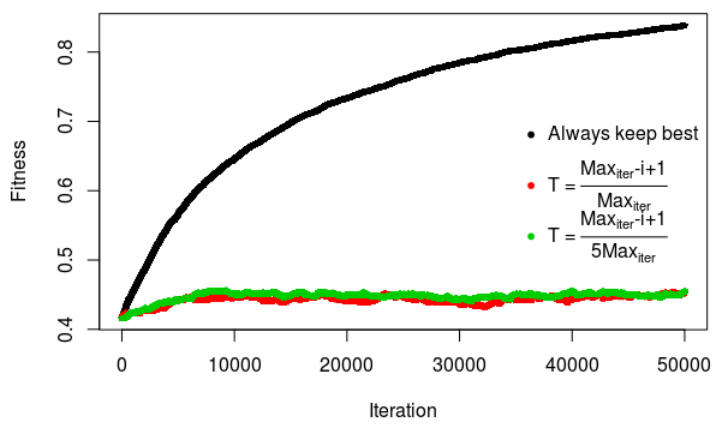
Figure 3.11 – Resulting fitness from Simulated Annealing with naive linear temperature function
