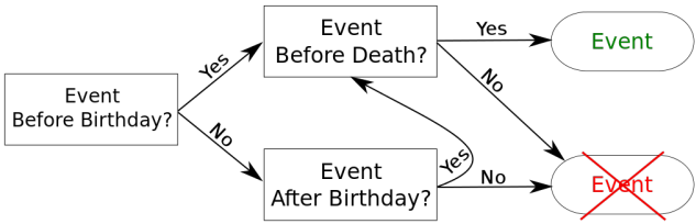
Figure 4.14 – Flowchart of the new method.
