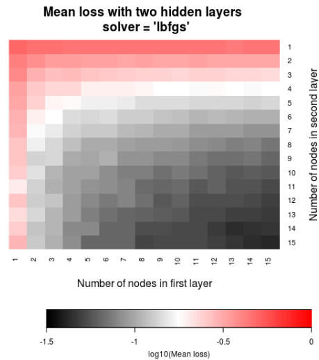
Figure 5.6 – Comparing the loss with two hidden layer, depending on the width of each layer
