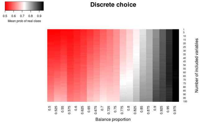
Figure 5.10 – Mean probabilities of real class depending on the number of inserted variables and the balance proportion between classes for discrete choice model.
