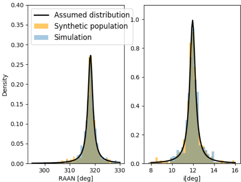
Figure 2.7 – Distribution of RAAN and inclination for the simulation and the synthetic population.
