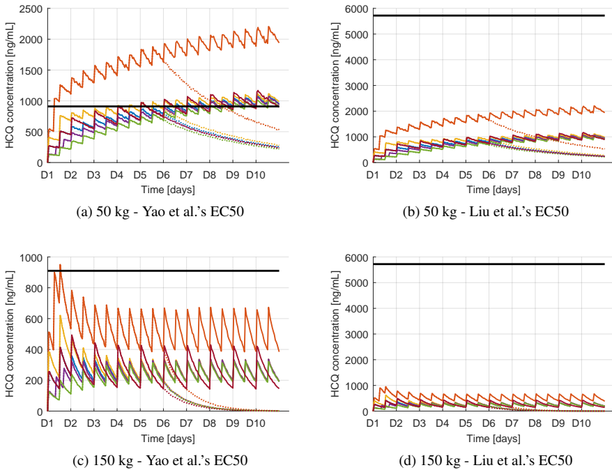
Figure 5.1 – Median PK profiles of HCQ blood concentrations after simulations ( n_{sim} = 1000 ) of alternative dosing regimens (see Table 5.1) for two representative patients of 50 kg and 150 kg, resp. The horizontal lines represent the projected target total whole blood concentrations based on the EC50 values from Yao et al. (2020) ( 0.72 \mu M ) and Liu et al. (2020) ( 4.51 \mu M ). Solid lines, treatment for 10 days; dotted lines, treatment for 5 days.
