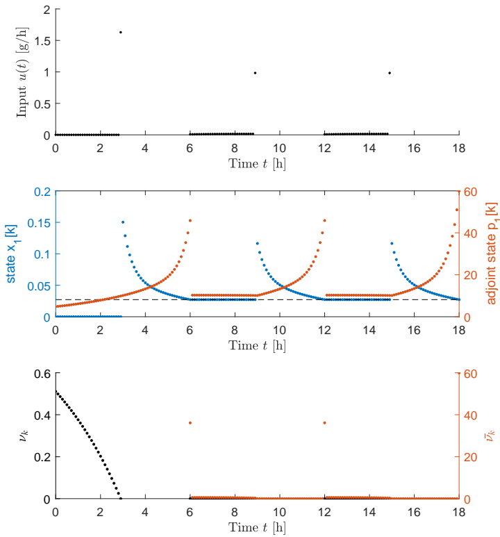
Figure 8.10 – Numerical resolution of the discrete-time L_1 -norm-based OC problem with constraint relaxation, using linprog.m ( j = 1, n_{\text{adm}} = 1 )
