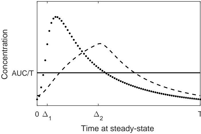
Figure 6.10 – Hypothetical PK profiles y_j^\infty(D, \Delta, T; \bar{t}) for different modes of administration, but equal dose. Dotted line, intermittent infusion ( \Delta = \Delta_1 ); dashed line, extended infusion ( \Delta = \Delta_2 ); continuous line, continuous infusion ( \Delta = T ).
