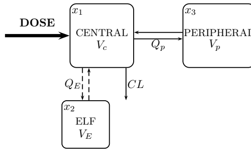
Figure 3.2 – Schematic representation of a (2+1)-compartment population pharmacokinetic model. CL , clearance; V_c , volume of distribution of the central compartment; Q_E , inter-compartmental clearance between the central and ELF compartments; V_E , volume of distribution of the ELF compartment; Q_p , inter-compartmental clearance between the central and peripheral compartments; V_p , volume of distribution of the peripheral compartment.
