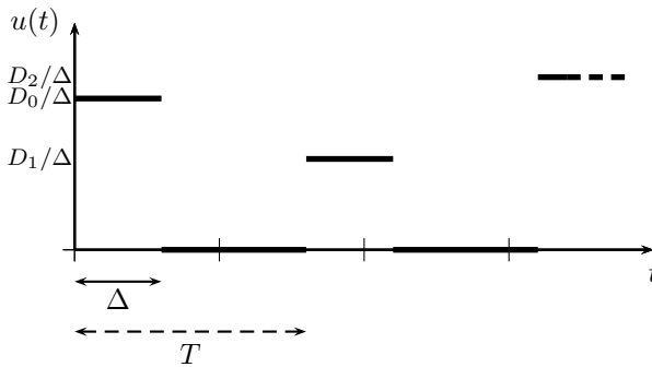
Figure 8.1 – System input function: drug infusion rate vs. time
