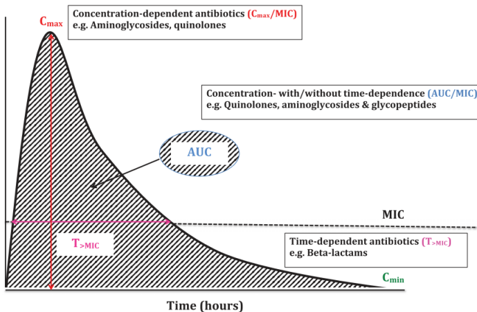
Figure 5.2 – Fundamental PK/PD indexes of antibiotics on a hypothetical concentration-time curve. AUC, area under the concentration-time curve; C_{\max} , maximal drug concentration; C_{\min} , minimum drug concentration; MIC, minimum inhibitory concentration; T_{>MIC} , time that drug concentration remains above MIC. Illustration taken from Abdul-Aziz et al. (2015).
