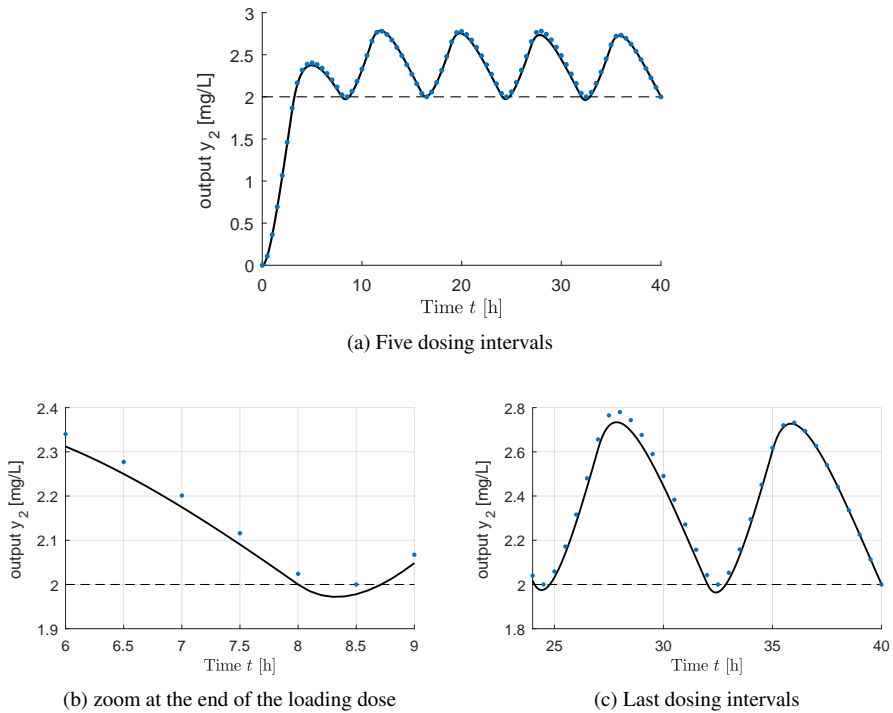
Figure 8.3 – PK profiles in ELF for different dosing strategies: continuous line, I/O approach with loading dose; blue points, OC approach in discrete-time setting using quadprog.m ( j = 2 , m = 5 ). The PK parameter Q_E was modified to amplify the time disconnect.
