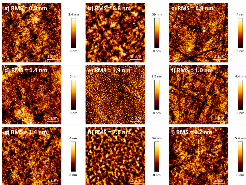
Figure 4. 10 \times 10 \mu\text{m} AFM images obtained for polymer solar cell devices made from a) PBDTT-TQxT:ITIC, b) PBDT2FT-TQxT:ITIC, c) PBDCIT-TQxT:ITIC, d) PBDTT-TQxT:PNDI(2OD)2T, e) PBDT2FT-TQxT:PNDI(2OD)2T, f) PBDCIT-TQxT:PNDI(2OD)2T, g) PBDTT-TQxT:PNDI(2OD)2T2Cl, h) PBDT2FT-TQxT:PNDI(2OD)2T2Cl, and i) PBDCIT-TQxT:PNDI(2OD)2T2Cl.
