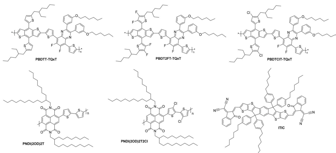
Fig. 1. Chemical structures of the donor polymers PBDTT-TQxT, PBDT2FT-TQxT and PBDDTCIT-TQxT, and the acceptors PNDI(2OD)2T, PNDI(2OD)2T2Cl and ITIC.
