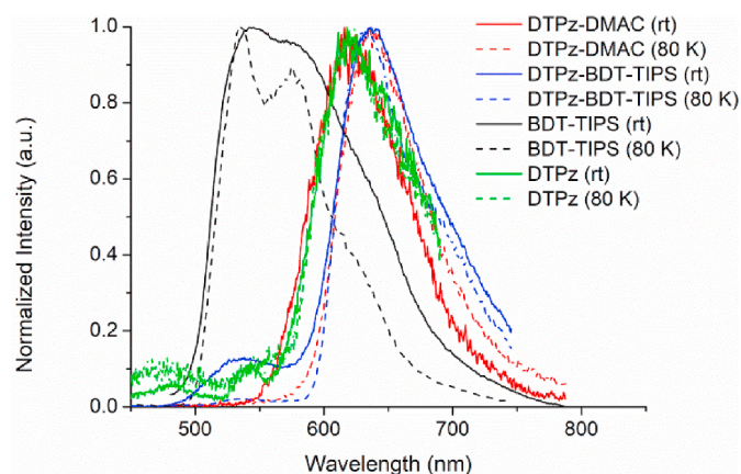
Fig. 4. Overlap of the emission spectra at 44.7 ms for DTPz-DMAC , DTPz-BDT-TIPS , DTPz and BDT-TIPS at room temperature and at 80 K in zeonex.
