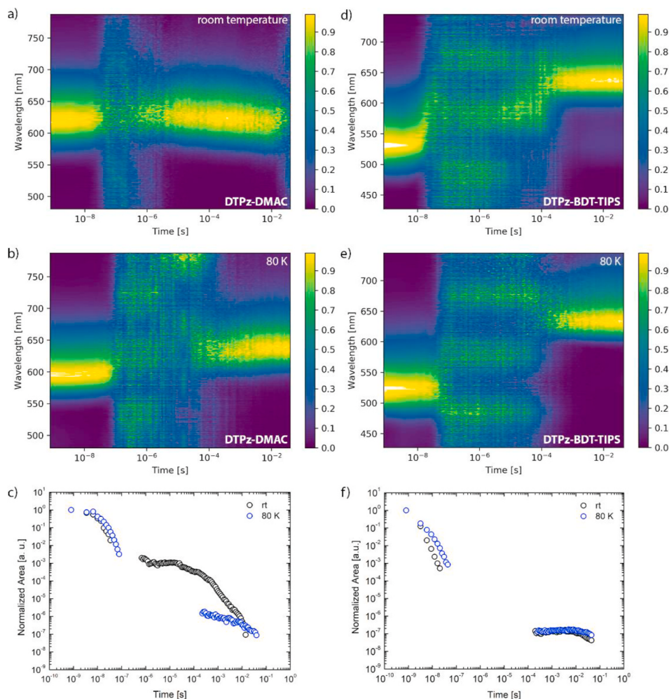
Fig. 3. Normalized time-resolved emission spectra for DTPz-DMAC (left) and DTPz-BDT-TIPS (right) in zeonex at room temperature (a,d) and at 80 K (b,e). Decays of the total emission for DTPz-DMAC (c) and DTPz-BDT-TIPS (f) at room temperature (rt) and at 80 K in zeonex.
