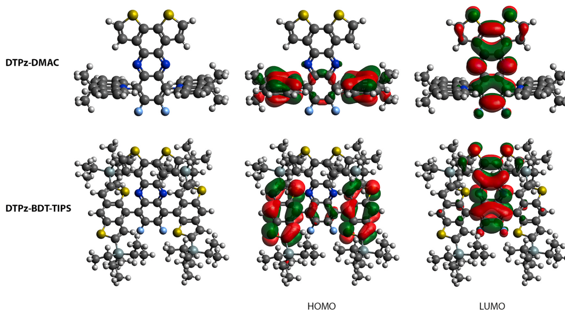
Fig. 1. HOMO and LUMO spatial distributions for DTPz-DMAC and DTPz-BDT-TIPS as obtained with LC-BLYP( \omega = 0.17 )/6-311G(d). Isocontour values of 0.02 (a.u.) were used for all orbitals.
