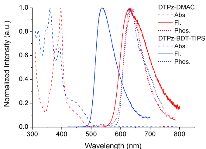
Fig. 2. Steady-state absorption (dashed lines) and emission (full lines) spectra at room temperature and time-resolved emission at a 44.7 ms delay time at 80 K (dotted lines) in zeonex film for DTPz-DMAC (red) and DTPz-BDT-TIPS (blue).
