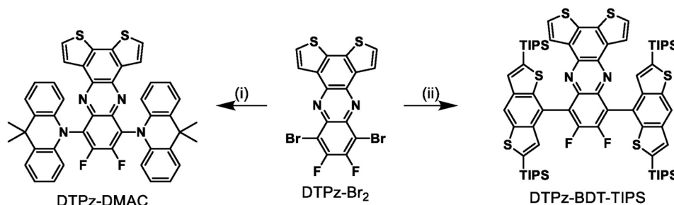
Scheme 1. Synthesis pathways toward DTPz-DMAC and DTPz-BDT-TIPS (TIPS = triisopropylsilyl): (i) 9,9-dimethyl-9,10-dihydroacridine, Pd(OAc) 2 , XPhos, NaOtBu, toluene, 110 °C, 24 h; (ii) BDT-TIPS-pinacol, Pd(PPh 3 ) 4 , K 2 CO 3 , DMF/H 2 O 4/1, 130 °C, 24 h.
