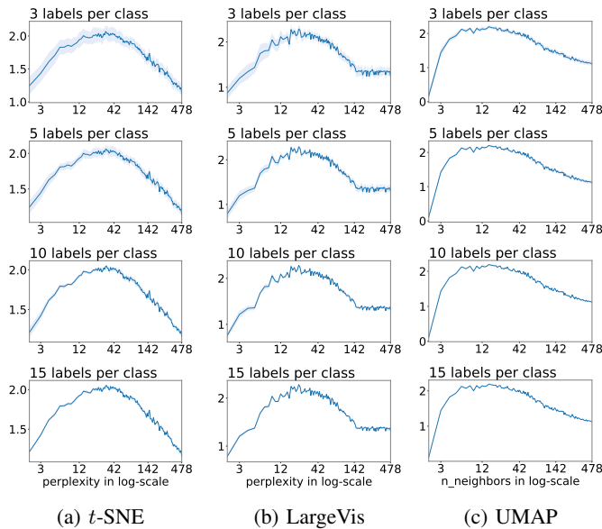
Fig. 5: Stability of f_{\text{score}} with the embeddings of (a) t -SNE, (b) LargeVis and (c) UMAP for the COIL20 dataset. The mean (blue line) and variance (filled region around the line) is calculated for each perplexity/ n_{\text{neighbors}} with a different number k of labeled instances per class (3, 5, 10 and 15).
