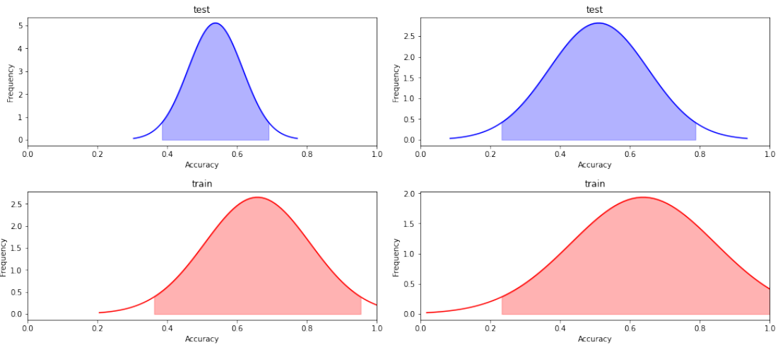
(a) Confidence interval for the generated ar- (b) Confidence interval for the generated ar- chitecture type LENET architecture type ALL
