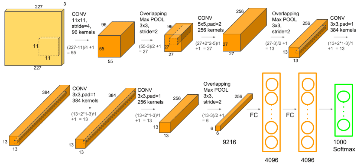
Figure 5.2: AlexNet architecture [41]
