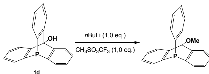
Scheme 17: Proposed synthesis for the methylation of the 9-phospha-10-hydroxytritycene.
