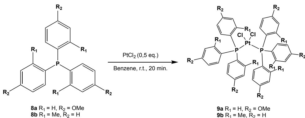
Scheme 11: Reaction of the reactions used to obtain soluble triarylphosphines Pt-complexes.
