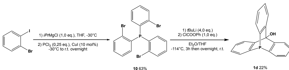
Scheme 12: Synthesis pathway to obtain the 9-phospha-10-hydroxytriptycene.
