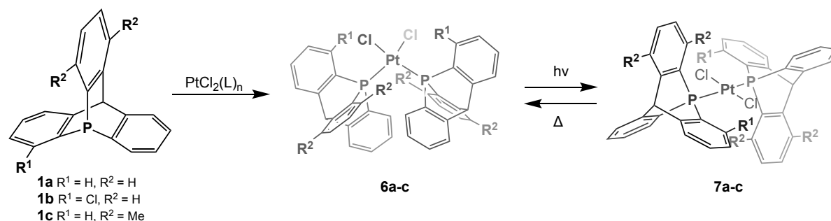
Scheme 5: Reaction of complexation on a PtCl_2 metal precursor.
