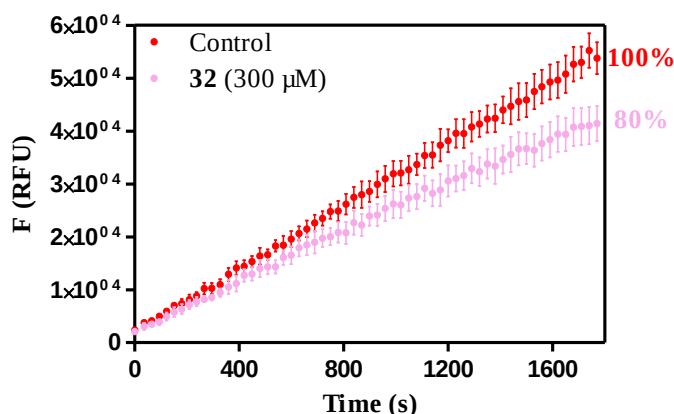
Figure 18 - Enzymatic activity of hUCH-L1 in the presence Benserazide 32 at 300 \mu M. No modulator (control) was defined as 100% activity.
