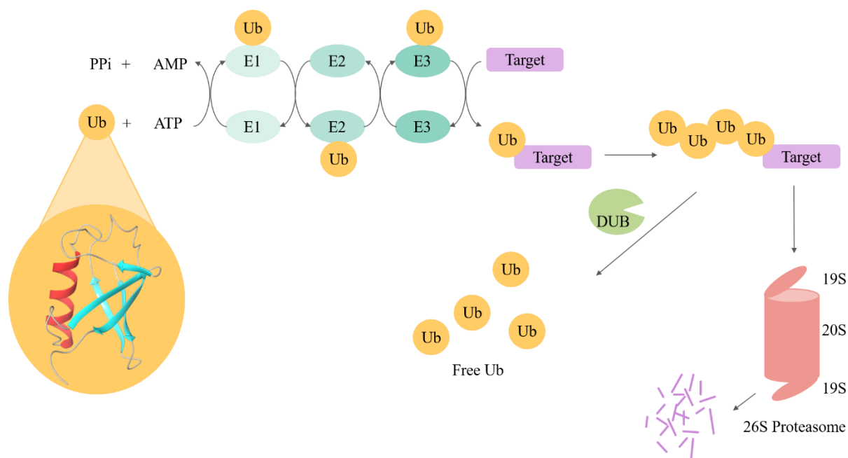
Figure 2 - Overview of the UPS. The binding of Ub to the protein target involves the sequential actions of E1, E2 and E3 enzymes in an ATP-dependent manner. Ubiquitinated protein target is recognized by the 19S unit of the 26S proteasome. DUBs enzymes remove Ub from the protein target which will be degraded into amino acids or peptides.
