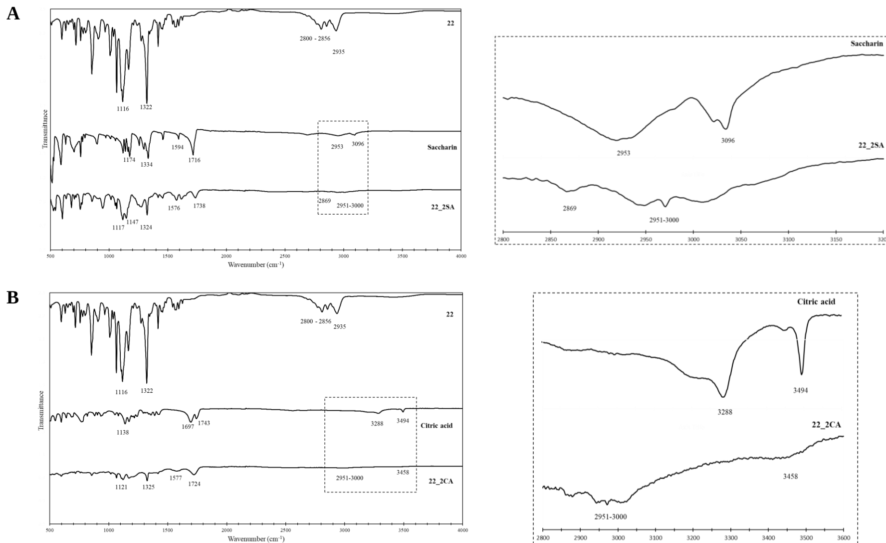
Figure 32 - IR spectra of (A) compound 22, saccharin and 22_2SA (from top to bottom) and of (B) compound 22, citric acid and 22_2CA (from top to bottom). Both followed of a magnification in the 3000 cm -1 regions.
