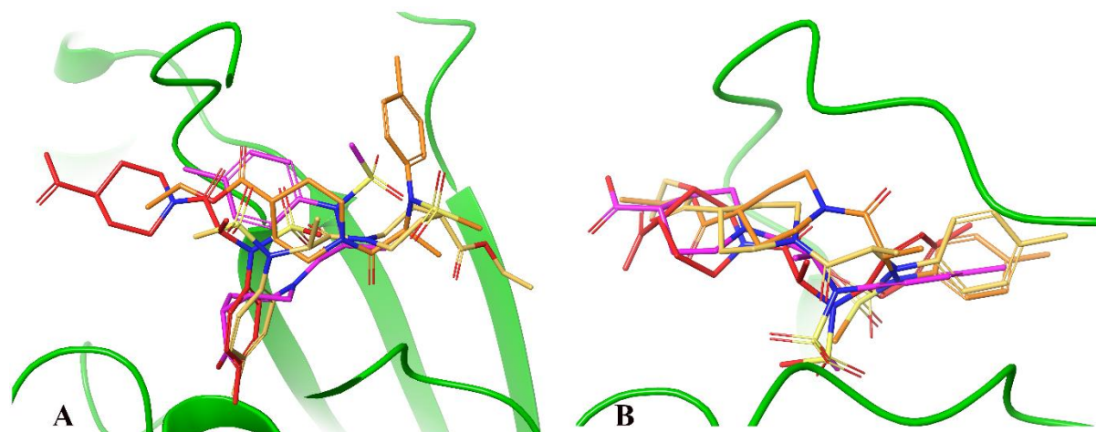
Figure 27 - Docking poses of (S) - 21 (orange), (R) - 21 (yellow), (S) - 36 (red) and (R) - 36 (purple) in the active site of hUCH-L1 inactive form (PDB: 2ETL, in green). Hydrogen atoms are not shown for clarity purpose. A: The best poses based on the glide score are presented for each compound. B: Based on the glide score: pose 3 of (S) - 21 , pose 4 of (R) - 21 and poses 2 of (S) - 36 and (R) - 36 are presented.
