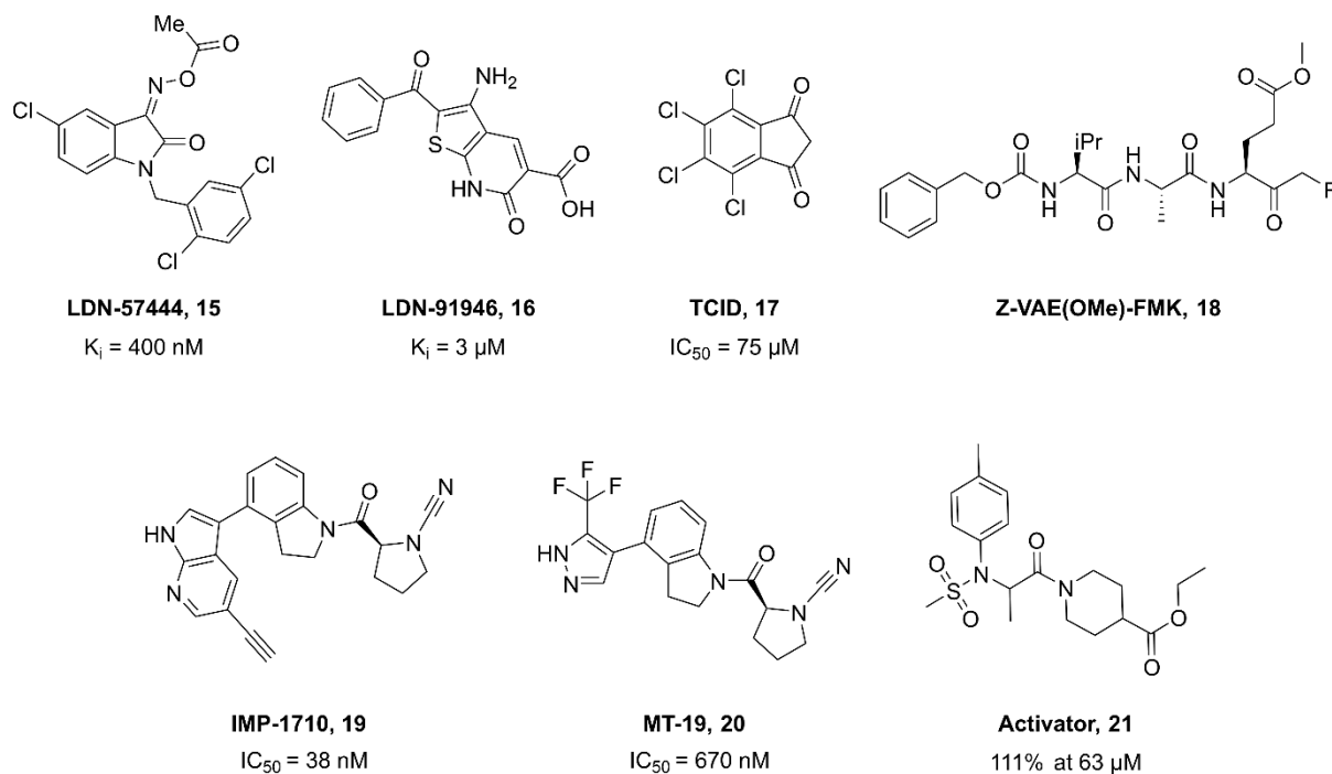
Figure 9 - Structure of selected UCH-L1 inhibitors and activators.
