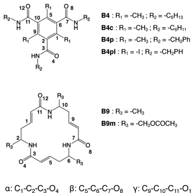
Fig. 1 Representation of the structures of the four molecules of the B4s family, B4 , B4c , B4p and B4pl and of the two molecules of the B9s family, B9 and B9m . The three important dihedral angles are also defined.
