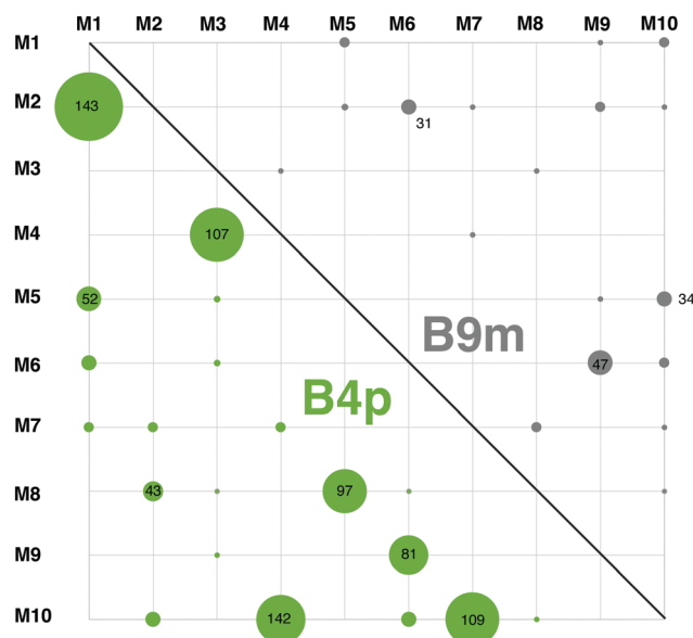
Fig. 12 Schematic representation of the occurrence of the formation of H-bonds between all the monomers ( M_i with i = 1 \dots 10 ) for B4p (bottom left, green) and B9m (up right, gray). The structures that are considered for the count are the final ones obtained at the end of the 1 ns simulation. The size of the dots is proportional to the number of H-bonds that have been detected. For the largest dots, we provided the corresponding exact number of interactions.
