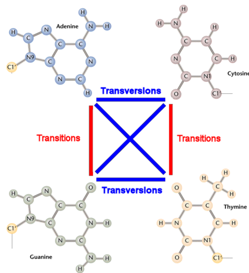
FIGURE 2.2.1 – Transversions vs transitions
