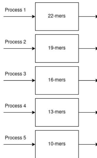
FIGURE 3.2.10 – Calcul de multiples k-mers de manière concurrente
