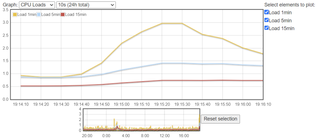
Figure 4.8: CPU Load
