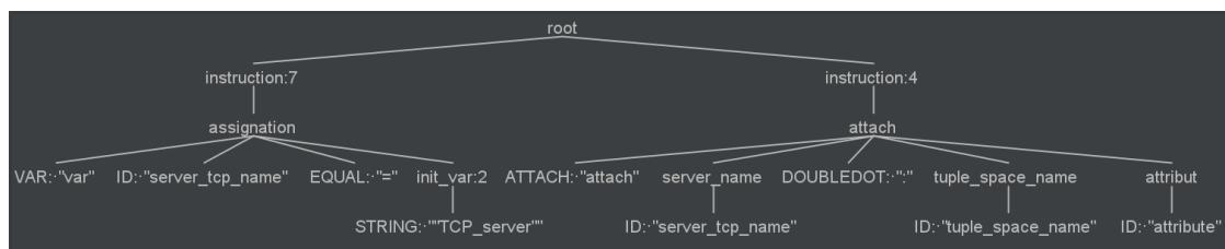
Figure 4.5: Parse tree.
