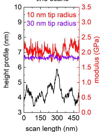
Fig. 4 Nanoscale mechanical properties and nanomechanical homogenization with time. a Topography and elastic properties (stiffness, adhesion, and modulus) in C16-IDTBT on the microscale. b Topography and elastic properties (stiffness, adhesion, and modulus) in C16-IDTBT on the nanoscale. The thin films were processed under identical conditions as those used in the electrical and thermoelectric devices but were left undisturbed under ambient conditions and in the dark for several weeks to allow the low molecular weight solvent molecules to evaporate from the surface under their own volatility. c Line scan of the modulus and topography along the dotted white lines shown in (b) measured using a tip radius of 10 nm. A scan of the modulus with a tip radius of 30 nm is shown in purple for comparison 63 . d Comparison of modulus histograms measured with two different tip radii; a 30 nm tip radius (larger than ordered film features) and a 10 nm tip radius (equivalent or less than ordered film features). e Comparison showing how the film adhesion changes far slower with time than the saturation mobility. f Normalized modulus measured on different C16-IDTBT samples using two different AFMs. The black dots correspond to the measurements on a Park Systems NX20 and the red dots correspond to measurements on a JPK NanoWizard 3 Atomic Force Microscope. The modulus reduction and homogenization that accompanies the reduction in adhesion force takes place on a time scale longer than the stabilization of the saturation mobility.
