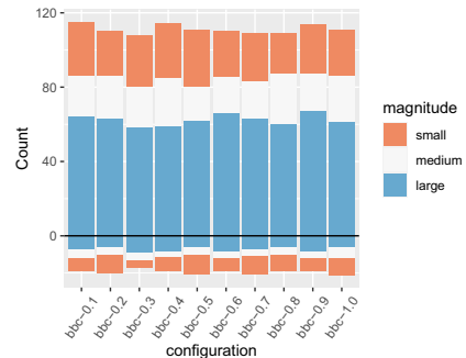
(b) \hat{A}_{12}(BBC_{Pr}, DYNAMOSA) magnitudes with a positive (count > 0 ) and negative (count < 0 ) effect and a p -value < 0.01
