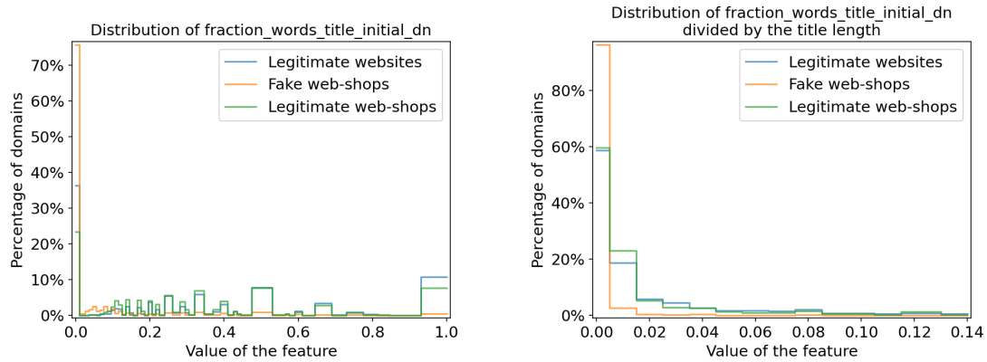
(a) Distribution of the fraction_words_title_initial_dn computed on the baseline dataset.
