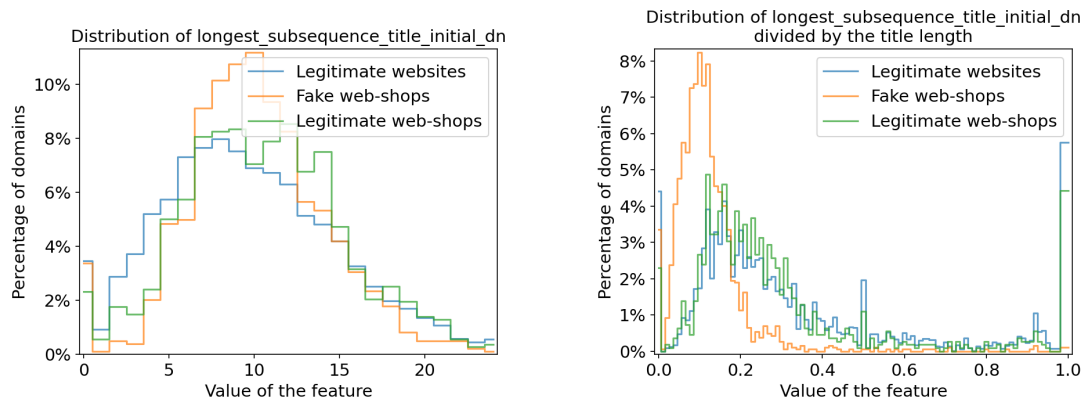
(e) Distribution of the longest_subsequence_title_initial_dn computed on the baseline dataset.
