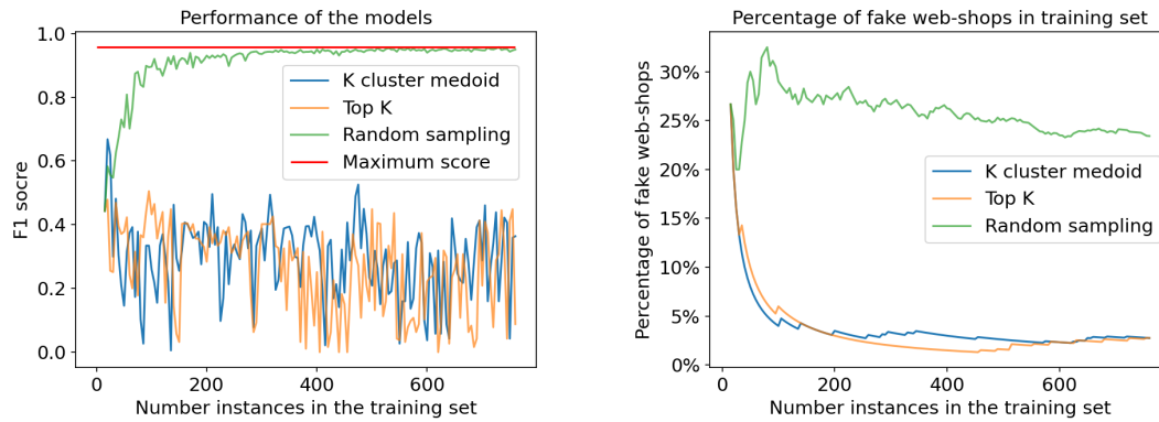
(a) F1 score of the different learners as more instances are added in their training set.
