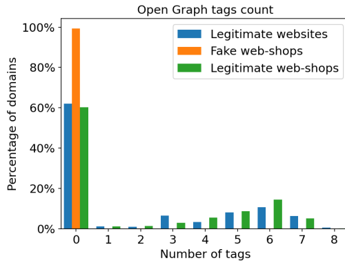
Figure 4.1: Almost none of the fake web-shop in our baseline dataset use Open Graph tags on the front page, while around 40% of legitimate websites do.
