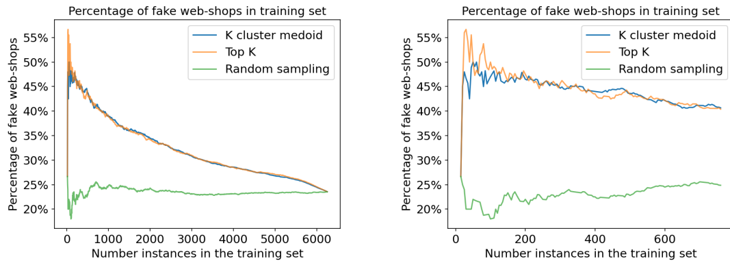
(a) Percentage of fake web-shops in the labeled dataset of the learners across all the iterations.
