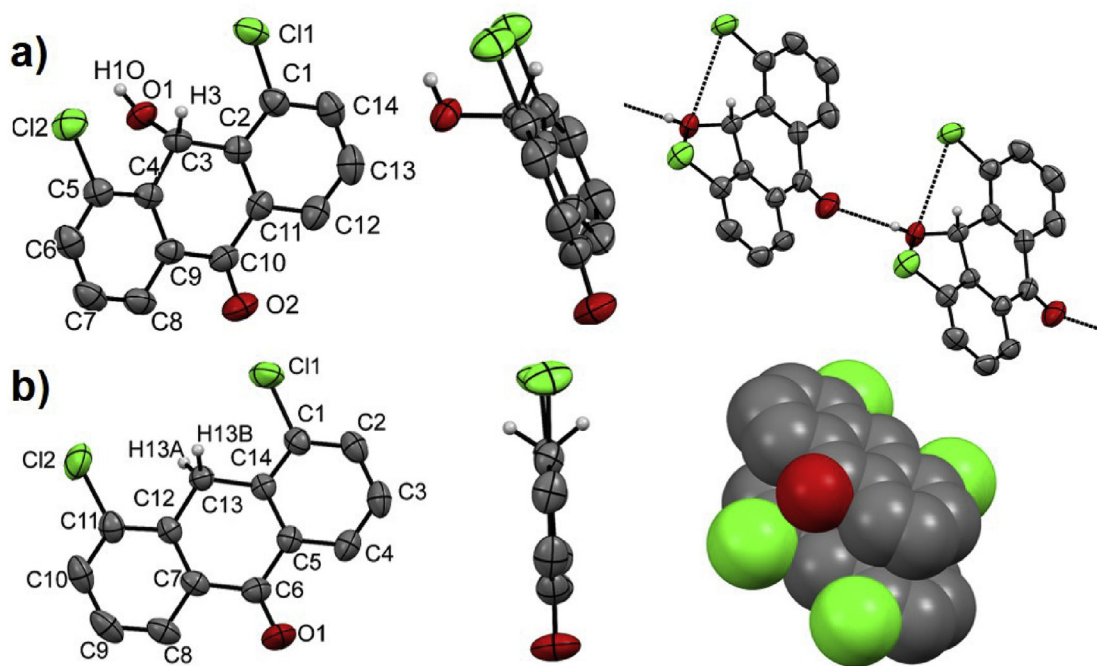
Fig. 5. a) Crystal structure of compound 13 ; space group: P2_1/c . b) Crystal structure of compound 10 ; space group: P-2_1 . H atoms are omitted except for OH and \text{Csp}_2\text{H} . Atom colours: green Cl, red O, grey C, white H.
