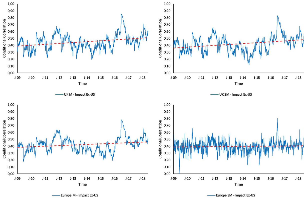
Fig. A3. Dynamic Conditional Correlation (DCC) between the Impact Investing Index (Ex-US) and the four MSCI benchmark indices ('J-09' stands for 'January 2009').
