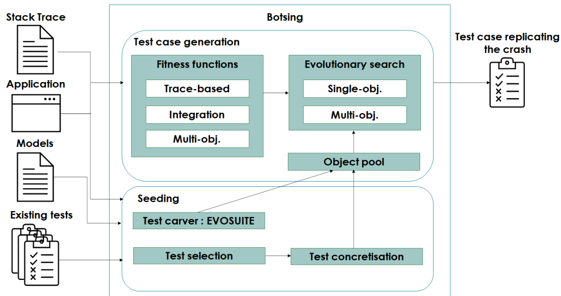
Figure 14: Architecture de Botsing[10]
