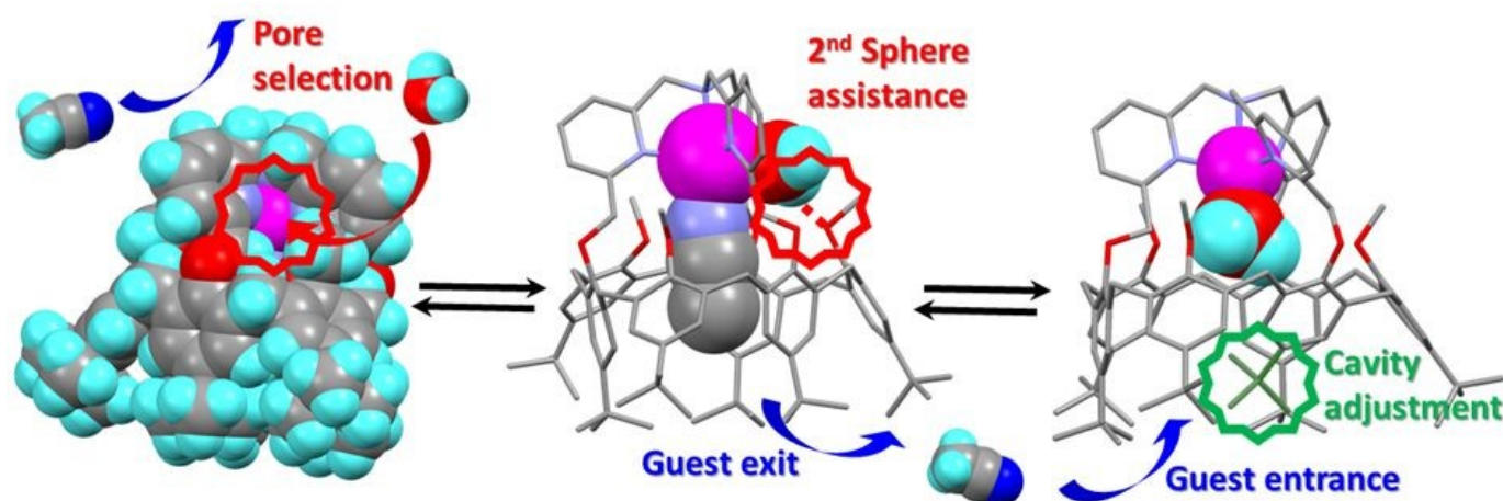
Figure 6. Key steps for the guest exchange catalyzed by a water molecule evidencing: (left) Pore-size selection for the exo-access to the metal center; (center) H-bonding assistance for the water ligand flipping from an exo to an endo position; (right) t Bu partial insertion for filling the cavity space.
