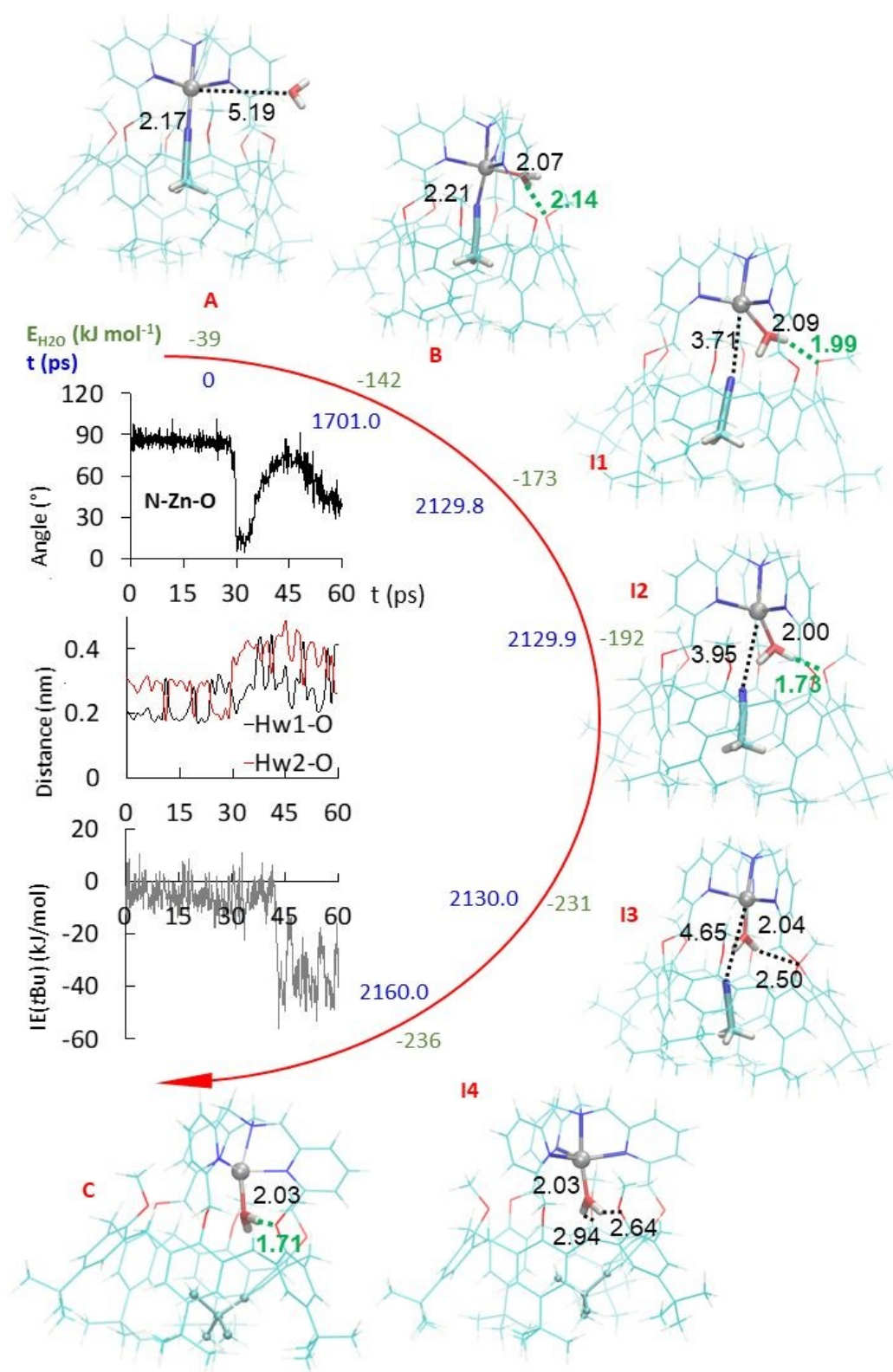
Figure 5. Stepwise substitution of MeCN guest by a water molecule following an associative pathway, as obtained from the 2,160 ps MD and SMD trajectories in vacuum at 300 K. Initial optimized structure - A, snapshot at 1,701 ps of the MD trajectory (coordination of H 2 O - B), at t = 29.8 of the SMD trajectory (insertion stage - I1), 29.9 ps (insertion stage - I2), 30.0 ps (insertion stage - I3), and 60.0 ps (final structure - I4). Semi-empirical MP7 optimized structure (C). Dotted lines refer to selected interatomic distances (in Å). Green dotted lines depict hydrogen bonds. The folded tBu moiety is displayed using ball and stick representations in I4 and C. Inset from top to bottom (obtained from the 60 ps long SMD trajectory): Variation of the NMeCN- Zn II -Owater angle and Hwater...OME distances; tBu-calixarene short-range interaction energy profile.
