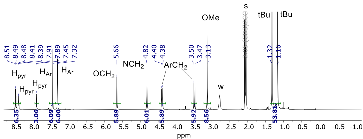
Figure S1. 1 H NMR spectrum (500 MHz, 300 K) of [Zn(H 2 O)L](ClO 4 ) 2 in acetone-d 6 .
