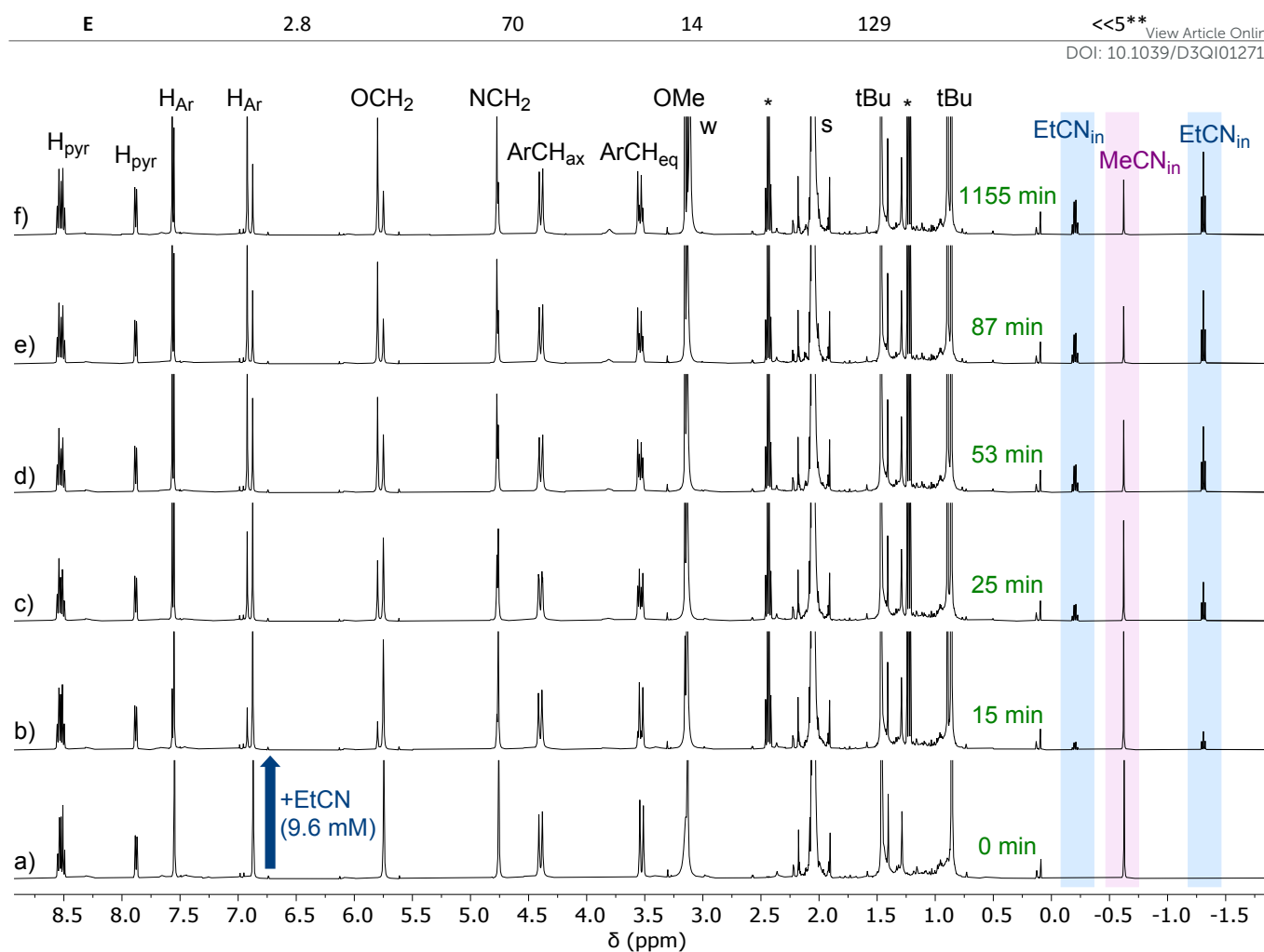
Figure 2. ^1\text{H} NMR spectra (300 K, 500 MHz, acetone- d_6 ) recorded during the titration of G = \text{MeCN} by G' = \text{EtCN} . Initial conditions in a) [\text{Zn}(\text{MeCN})\text{L}]^{2+} = 3.7 \text{ mM} , [\text{free MeCN}] = 92 \text{ mM} , [\text{EtCN}] = 0 \text{ mM} , [\text{H}_2\text{O}] = 20 \text{ mM} . Percentage of EtCN complex in solution: a) 0%, b) 17%, c) 38%, d) 41%, e) 59%, f) 71%. This experiment is reported as entry A in Table 1. Full conversion corresponds to the amount of EtCN complex formed at equilibrium under these experimental (71%). The “t(50% conversion)” is then the time at which we have 35.5% of EtCN complex in solution. *: free EtCN.
