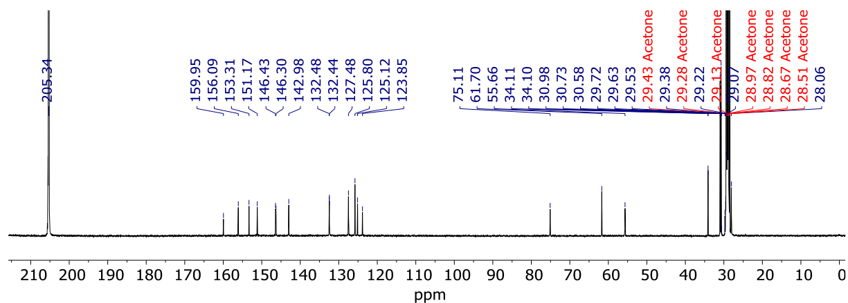
Figure S2. 13 C NMR spectrum (126 MHz, 300 K) of [Zn(H 2 O)L](ClO 4 ) 2 in acetone-d 6 .
