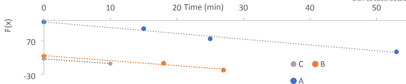
Figure 3. Kinetic fit of the ^1\text{H} NMR analyses. For the expression of F(x) , see (Eq. 4). A,B,C refers to experiments of Table 1.
