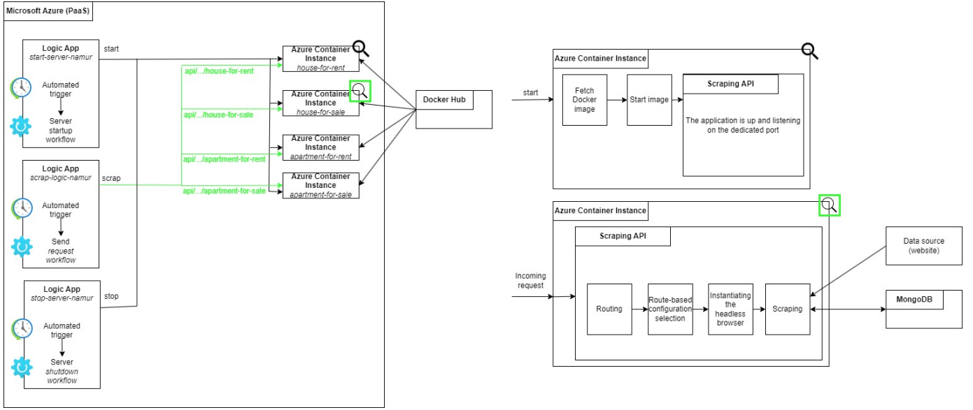
Fig. 2. The cloud architecture used to deploy SCRIMMO
