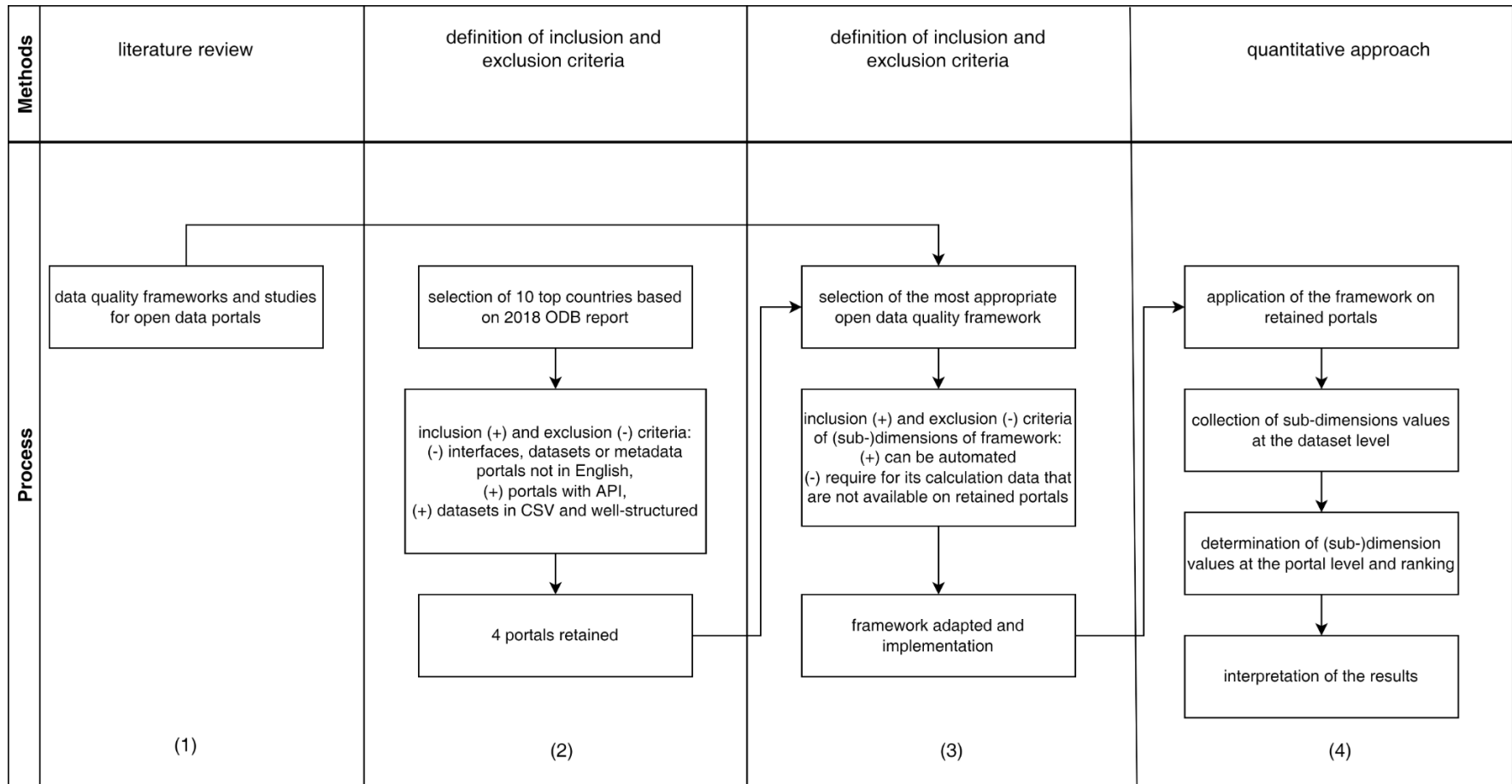
Figure 1: Research methodology.
