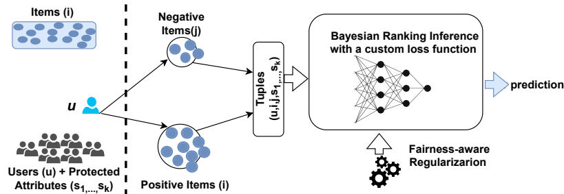
Figure 1: The FairBayRank system model.
