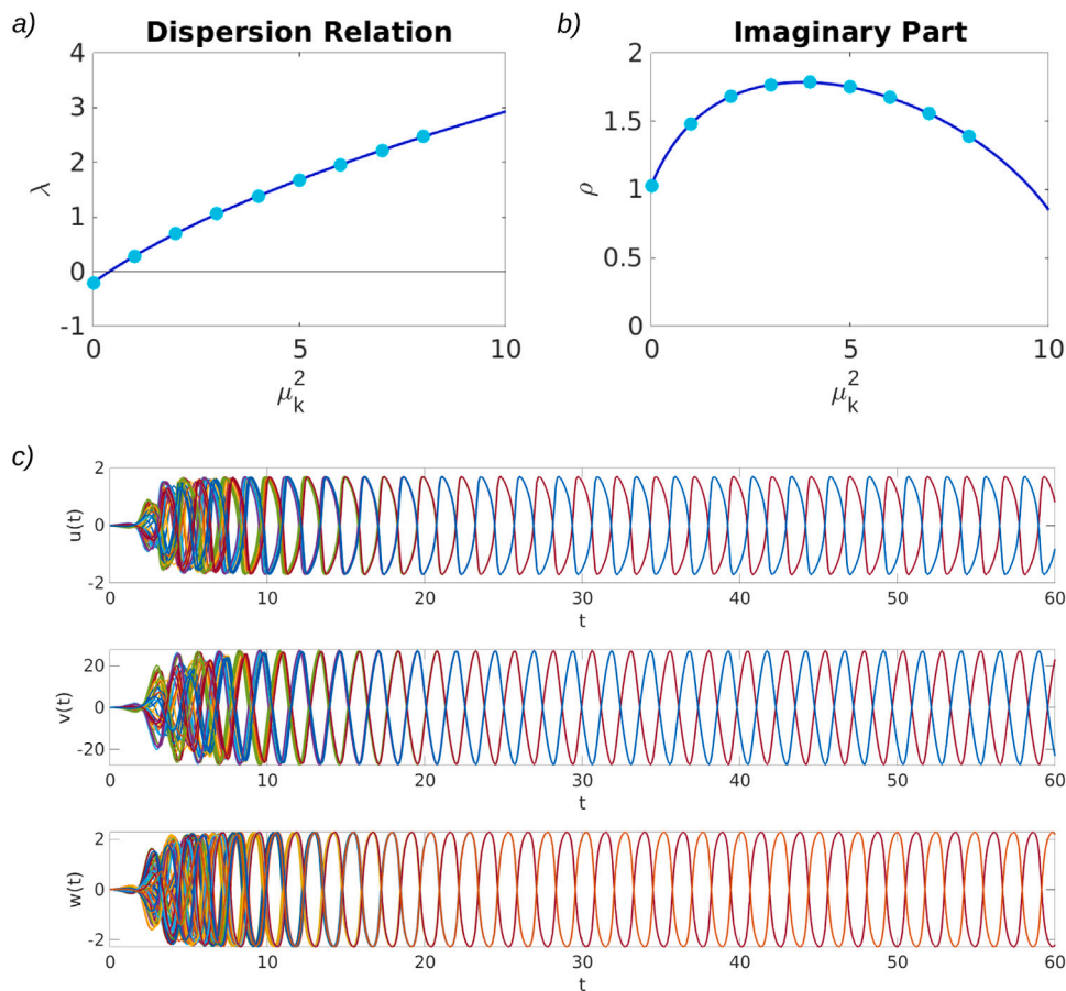
Fig. 5. Dispersion relation and Dirac-induced patterns Panel (a) shows the real part of the dispersion relation \lambda , while panel (b) its respective imaginary part \rho . The dispersion relation is computed as for the case with diffusion (Fig. 3, panels a and b). We can observe that the real part of the dispersion relation is divergent, however this does not pose a problem given that our support is discrete and finite, and so is its spectrum. The chosen setting is such that Dirac-induced patterns emerge ( \lambda > 0 ) and they are oscillatory (the corresponding \rho \neq 0 ), as shown by the dynamics of the 3 interacting species, in panel (c). The network is a 2D lattice with periodic boundary conditions of 36 nodes and the parameters are \sigma_1 = 1 , \sigma_2 = -1.4 , \sigma_3 = -10 , \eta_1 = -3 , \xi_1 = -0.5 , \xi_2 = 5 , \zeta_1 = 0.1 , \zeta_2 = 6 , \zeta_3 = 6 , \zeta_4 = 1 , c_1 = -1 , c_2 = 0 , \alpha_u = 1 , \alpha_v = 1 , \beta_u = 1 , \beta_v = 0.1 ; the initial perturbation is the order of 10^{-2} .
