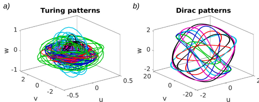
Fig. 11. Projected attractors (a) Turing patterns, (b) Dirac-induced patterns. The network is the Random Eulerian Network of Fig. 8. (a) The parameters are \sigma_1 = 0.3, \sigma_2 = -2, \sigma_3 = -2, \eta_1 = -3, \xi_1 = -0.5, \xi_2 = 5, \zeta_1 = 0.1, \zeta_2 = 6, \zeta_3 = 6, \zeta_4 = 1, c_1 = -1, c_2 = 1, \alpha_u = 1, \alpha_v = 1, \beta_u = 1, \beta_v = 0.1 . (b) The parameters are \sigma_1 = 0.3, \sigma_2 = -2, \sigma_3 = -10, \eta_1 = -3, \xi_1 = -0.5, \xi_2 = 5, c_1 = -1, \alpha_u = 1.1, \alpha_v = 7, \beta_u = 7, \beta_v = 1.1 ; the initial perturbation is the order of 10^{-2} .
