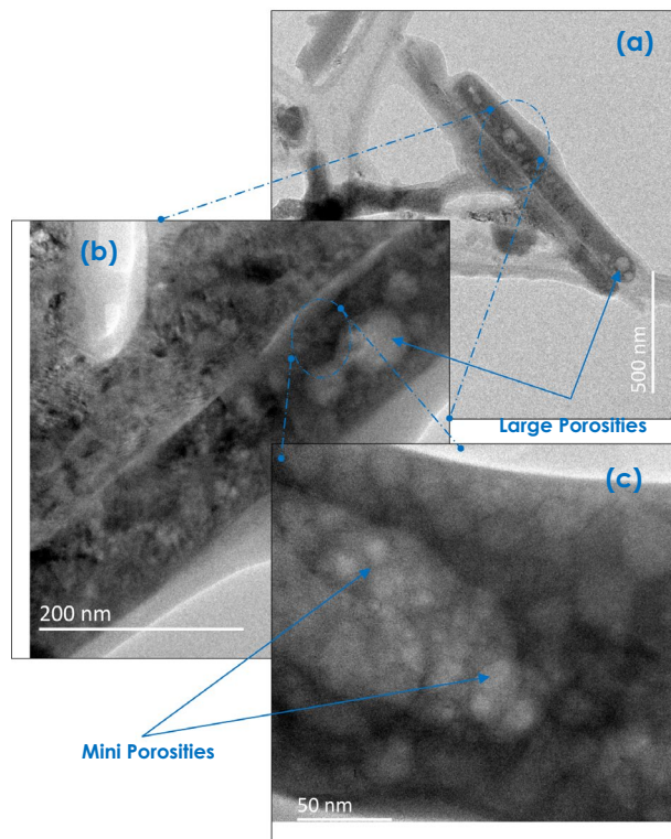
Figure 10. Multi-scale porosity in the bio-engineered \text{CaCO}_3 1-D nanoparticles.
