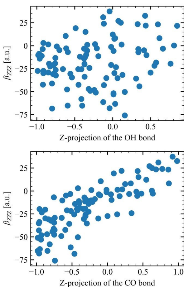
Figure 5. Correlation between the \beta_{ZZZ} response and the orientation of the OH (top) and CO (bottom) bond, as determined by their projections onto the Z axis.
