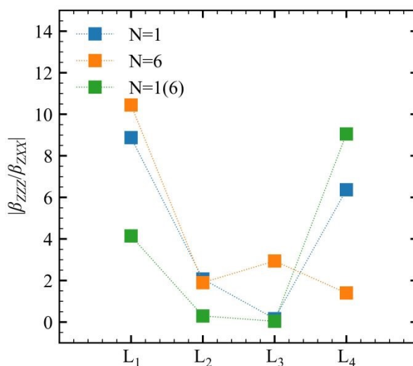
Figure 6. |\beta_{zzz}/\beta_{zxx}| ratio as a function of the molecular layer obtained at T = 300 K for different QC schemes. Note that the value obtained for N = 1(6) at L_4 is divided by 10 for clarity.
