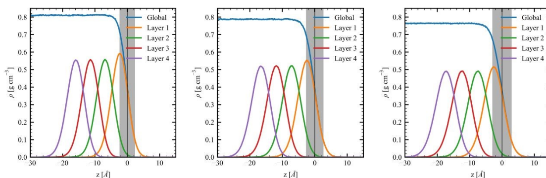
Figure 3. Interfacial density profiles for the MeOH slabs at (left) T=260 K, (center) T=280 K, and (right) T=300 K, as well as for its first four layers. The interfacial position (black vertical line) and interfacial roughness (gray shade) are also presented.
