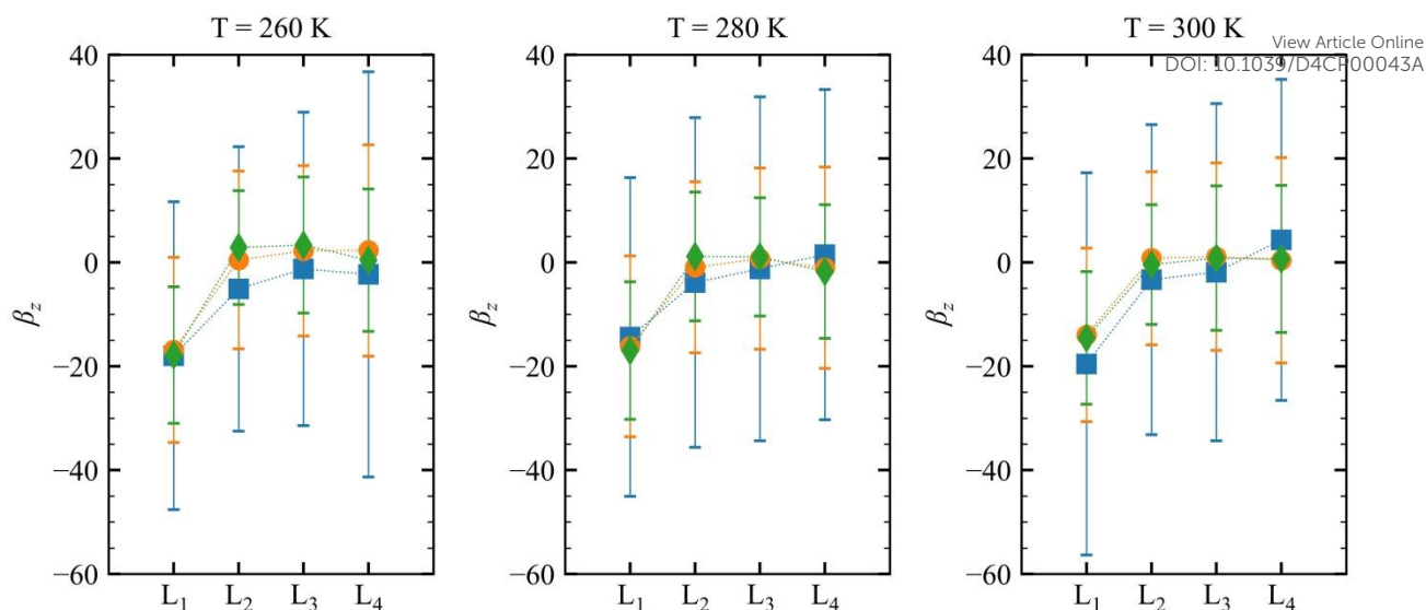
Figure 4. \beta_z values, as a function of the molecular layer, calculated at \lambda=1064 nm. The average values (per molecule) are represented by symbols (blue squares for N = 1 , orange circles for N = 3 , and green diamonds for N = 6 ), whereas the standard deviations are given by error bars.
