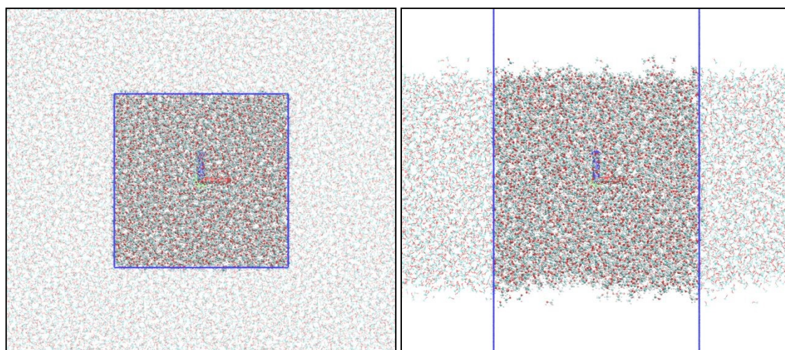
Figure 1. Snapshots from bulk (left) and slab (right) MD simulations. The blue lines identify the MD simulation boxes. The images were created using VMD. 36
