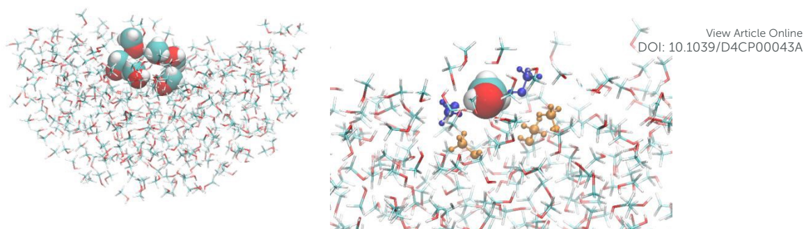
Figure 2. A snapshot illustrating the interfacial model used in the quantum chemical calculations. Left: a cluster with 6 MeOH molecules surrounded by 20 Å of polarizable embedding sites. Right: A detailed view of the cluster highlighting the central (vdW representation), the hydrogen-bonded (blue), and first neighbors (orange) MeOH molecules. The images were created using VMD. 36
