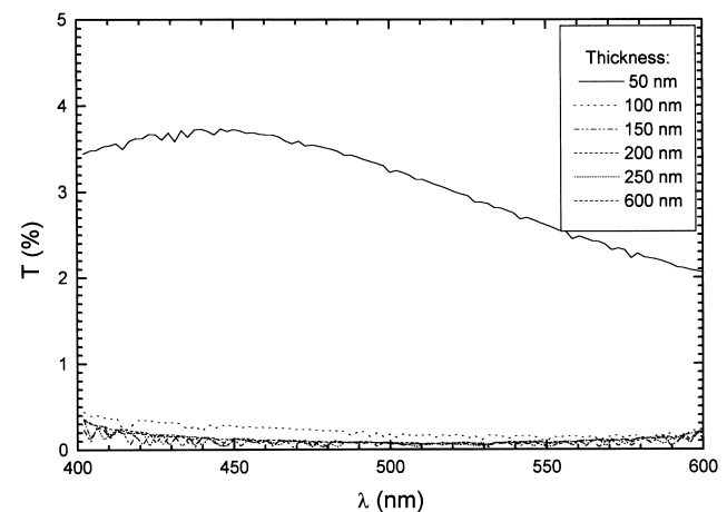
Fig. 1. Light transmission spectra T(\lambda) from 400 to 600 nm through six different TiN x film thicknesses deposited onto glass substrates (4 sccm N 2 , 0.30 Pa, 8 mA/cm 2 ).
