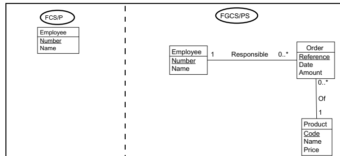
Fig. 11. The conceptual federated schemas. FCS/P integrates the LES of the personnel databases whereas FGCS integrates FCS/P and the LES of the sales department.
