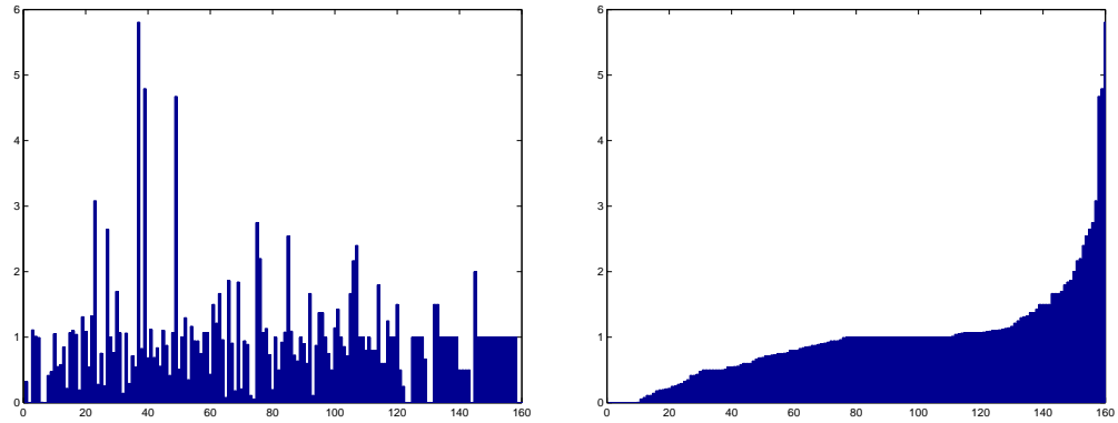
Figure 7.6: The reduction (or increase) of solution time with presolving in medium mode, sorted by decreasing solution time for the original problem (left) and by decreasing reduction (right).
