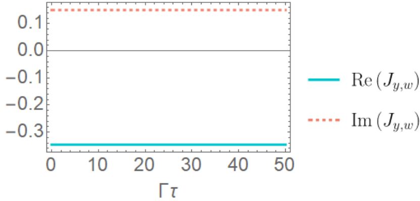
Figure B3. Real and imaginary parts of the weak value of \hat{J}_y as a function of the product of the dissipation time and the dissipation rate. The pre- and post-selected states are detailed in the text and are chosen to create a constant anomalous weak value.
