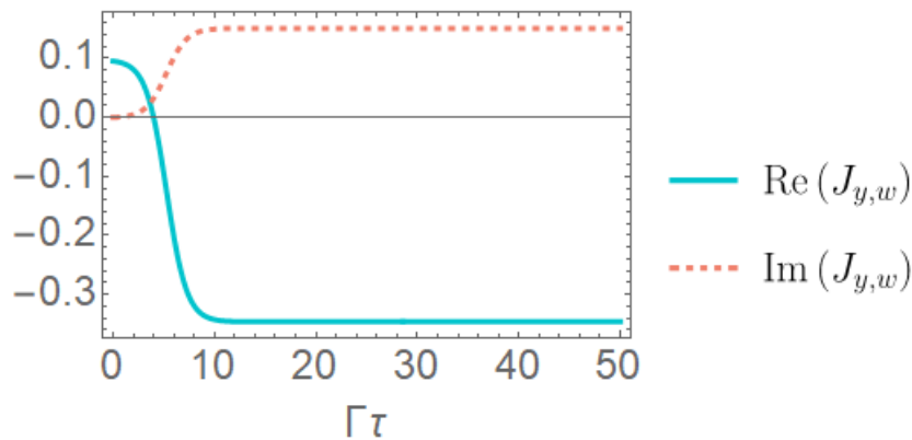
Figure B2. Real and imaginary parts of the weak value of \hat{J}_y as a function of the product of the dissipation time and the dissipation rate. The pre- and post-selected states are detailed in the text and chosen to illustrate the occurrence of an increasing anomaly due to dissipation.
