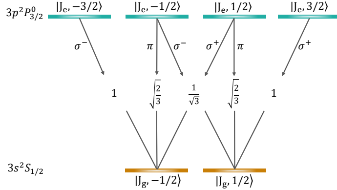
Figure B1. Atomic transition J_g = \frac{1}{2} \leftrightarrow J_e = \frac{3}{2} . The Clebsch-Gordan coefficients for each transition, C_{m_g, q, m_e}^{J_g, 1, J_e} = \langle J_g, m_g; 1, q | J_e, m_e \rangle are shown for each allowed transition.
