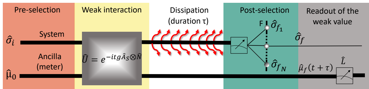
Figure 1. Overview of the steps involved in the dissipative weak measurement protocol. The process begins with pre-selection of the system, followed by the implementation of a weak measurement described through the unitary operator \hat{U} . After the weak interaction, the system undergoes dissipation for a duration \tau before a post-selection. Finally, the meter is readout to extract information on the weak value.
