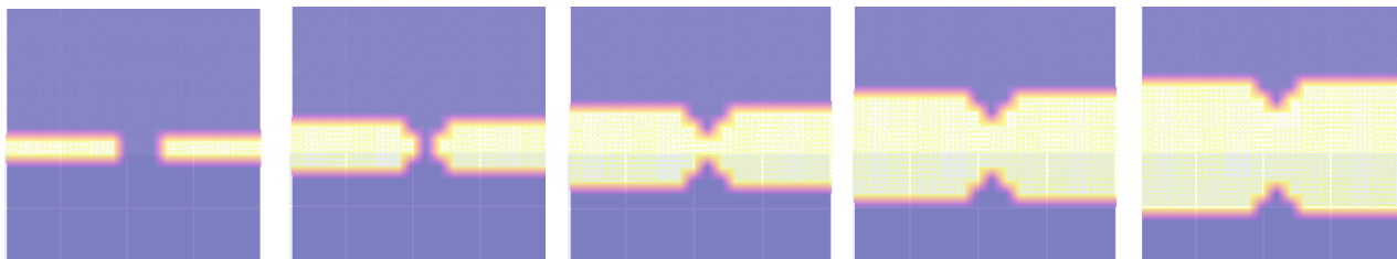
Figure 7: 1, 2, 3, 4, and 5-step (from left to right) empowerment levels, computed across the 2-D grid in condition W6 and projected on the X-Y plane. The placement of the obstacle exactly on the borderline between black and white regions explains the symmetry of the profiles and its detrimental effect on empowerment levels for all horizons.
