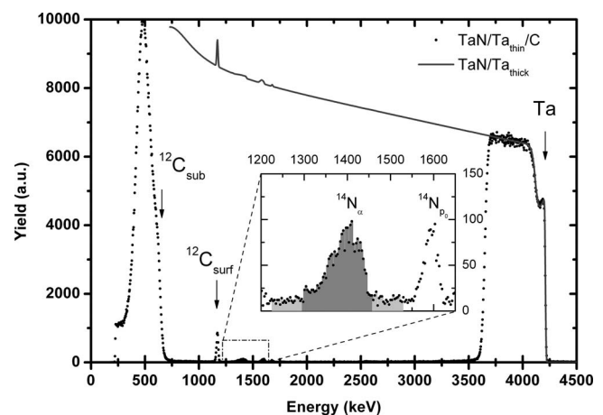
FIG. 1. Backscattering spectra for 4.6 MeV \alpha -particles observed at 165^\circ on TaN/Ta standards without absorber in front of the detector: experimental points on the thin Ta( ^{14}\text{N} )/C standard (dots) and simulation for TaN on a thick Ta backing (solid gray line). In insert, the mean of the background on the left and right of the reaction peak is subtracted from the nitrogen peak to calculate the cross-section. ^{14}\text{N}_\alpha and ^{14}\text{N}_{p_0} notations are for the ^{14}\text{N}(\alpha, \alpha)^{14}\text{N} and ^{14}\text{N}(\alpha, p_0)^{17}\text{O} reactions, respectively.
