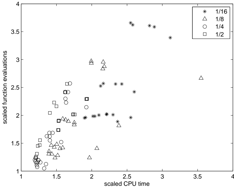
Figure 4.4: Average scaled function evaluations versus average scaled CPU-time for all algorithmic variants, distinguishing the values of \kappa_\chi .
