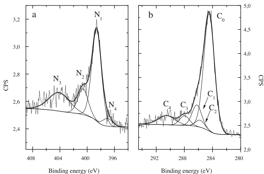
Fig. 3. N 1s (a) and C 1s (b) XPS spectra recorded at a 645 nm depth for the copper sample implanted with ^{13}\text{C} and ^{14}\text{N} at 250 °C. Experimental data are represented by short dot lines. Solid lines are the results of the curve fitting Gaussian–Lorentzian components and the sum of them.
