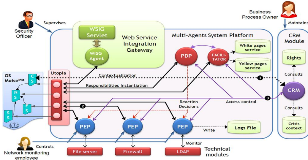
Figure 1. Synoptical ReD Architecture
