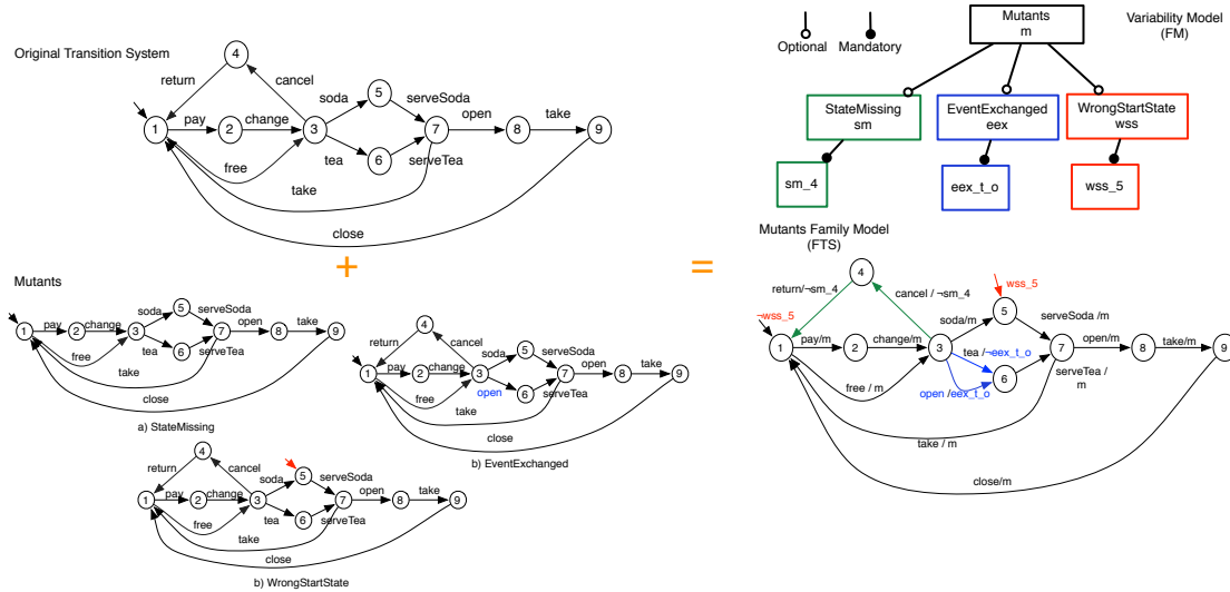
Figure 1: Approach Overview
