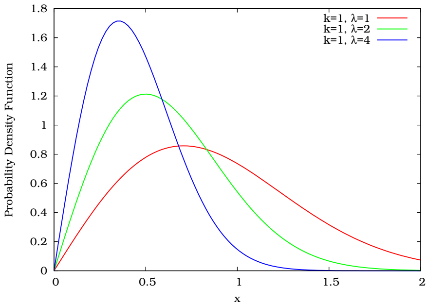
Figure C.7: Weibull distribution.
