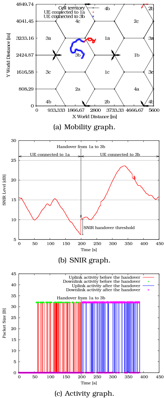
Figure 4.8: Handover impacts.
