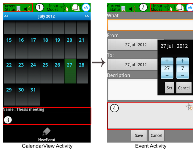
Figure 1. MAA user interface
