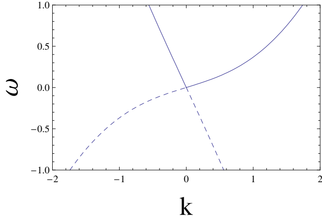
FIG. 1: Dispersion relation for subsonic configurations. The solid (dashed) line corresponds to the positive (negative) norm branch: \omega - vk = +(-)c\sqrt{k^2 + \frac{c\xi k^4}{4}} .
