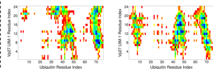
Fig. 6 Shortest contact map Vps27 UZM-1 - Ubiquitin (1QOW). (left) AT_V MD simulation, (right) all-atom MD simulation.
