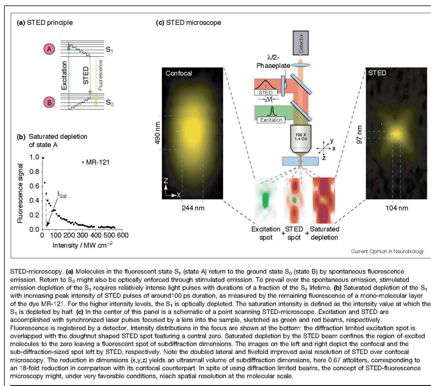
Fig. 2 : Microscope STED 7
