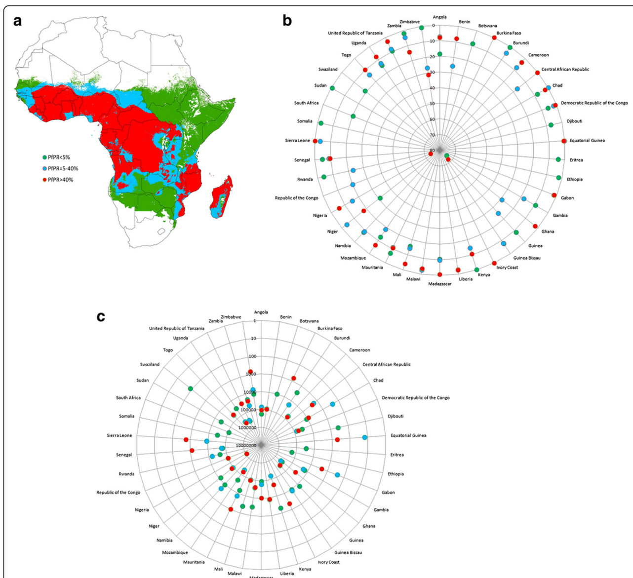
Figure 2 P. falciparum malaria prevalence in Africa and the effects on metrics of accounting for subnational age structure. (a) Predicted prevalence classes for P. falciparum malaria in Africa [5]. (b) The absolute percentage changes in estimated numbers of children under 5 years old residing under the three prevalence classes through changing from using UN national proportions [27] to produce per grid cell estimates of numbers under 5 years to using the subnational proportion data assembled here (Additional file 1: Protocol S1). (c) The changes in estimated numbers of children under 5 years old residing under the three prevalence classes through changing from using UN national proportions [27] to produce per grid cell estimates of numbers under 5 years to using the subnational proportion data assembled here (Additional file 1: Protocol S1). In (b) and (c) , data values are only plotted when a transmission class encompasses >10% of the population of a country.
