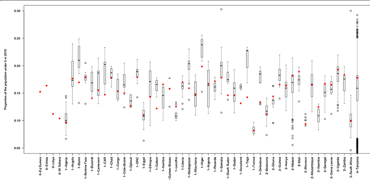
Figure 3 Differences between national and subnational summaries of population proportions under 5 years old for African countries. Comparison of UN national estimates [27] of proportions of the population under 5 years old in 2010 (red dots) against the range of proportions measured by the subnational datasets collated here (Additional file 1: Protocol S1) shown as boxplots. The solid center line of the boxplot shows the median values, the box width represents the interquartile range, and the whiskers extend to 1.5 times the interquartile range from the box (values further away than this are shown as open circles). The administrative unit level of the subnational data used here is shown as a prefix to the country name on the x-axis.
