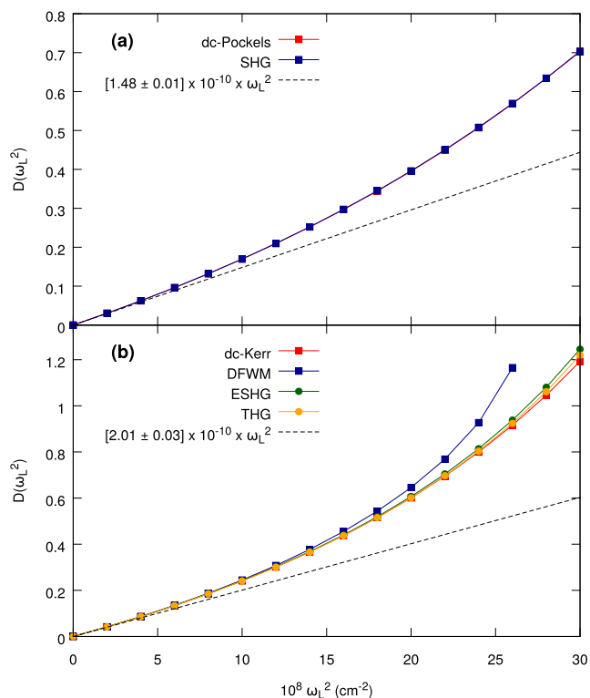
FIG. 4. CCSD/d-aug-cc-pVDZ frequency dispersion [D(\omega_L^2)] for \beta_{\parallel} (a) and \gamma_{\parallel} (b) of methanol for different second- and third-order NLO processes. The dashed line corresponds to Eq. (7) truncated at the second order.
