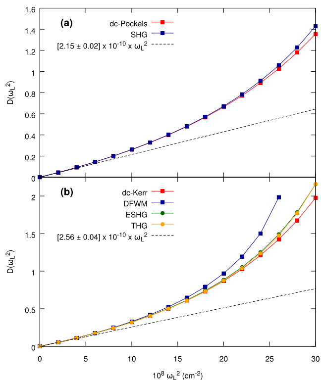
FIG. 5. CCSD/d-aug-cc-pVDZ frequency dispersion [D(\omega_L^2)] for \beta_{\parallel} (a) and \gamma_{\parallel} (b) of DME for different second- and third-order NLO processes. The dashed line corresponds to Eq. (7) truncated at the second order.
