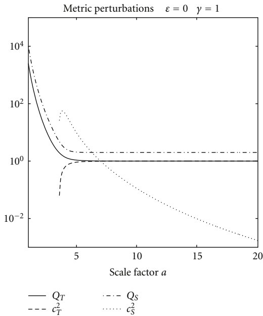
FIGURE 5: Evolution of the parameters for metric perturbations (scalar and tensorial parts), respectively, Q_S, c_S^2, Q_T, c_T^2 , as defined in the text versus the scale factor, for \gamma = 1 . As found theoretically, the initial high velocity of the field drives both the speed of (scalar and tensor) metric perturbations to imaginary values, thus signaling a breakdown of hyperbolicity for metric perturbations (here it happens when the corresponding curves terminate, since the y axis is in logarithmic scale).
