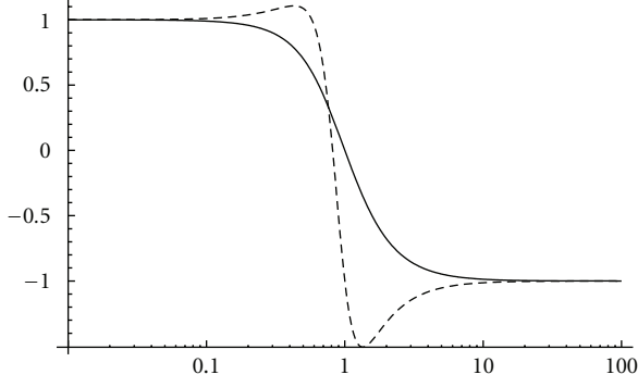
FIGURE 1: log linear plot of \omega_\phi as a function of the dimensionless variable \kappa\phi for \gamma = 1 and \gamma = -1 (dashed).
