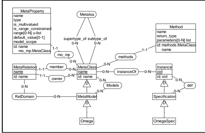
Fig. 1. Meta-Meta-Model This E/R schema shows the definition of our meta-meta-model. Technical details have been erased for pedagogic reasons. The Models and RelDomain relationships denote the possible constituents of a meta-model. The meta-relation instances are not shown, they have been hard-coded for efficiency purpose.
